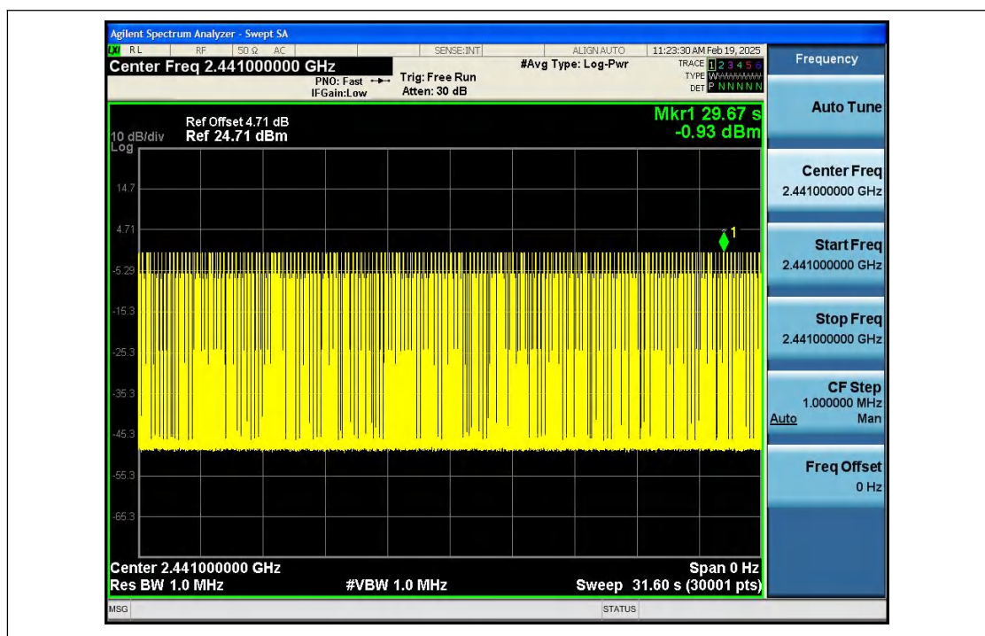
Dwell_Time_(Hopping)_NVNT_ANT1_3-DH3_2441_00_One_Burst_Time
