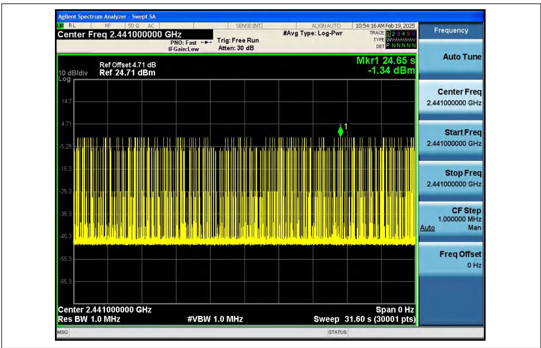
Dwell_Time_(Hopping)_NVNT_ANT1_3-DH5_2441_00_One_Burst_Time
