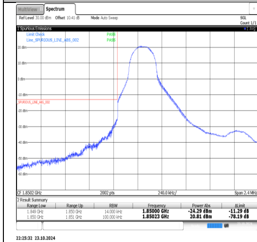
Band25-1.4MHz-QPSK-26047-1RB#5-PASS
