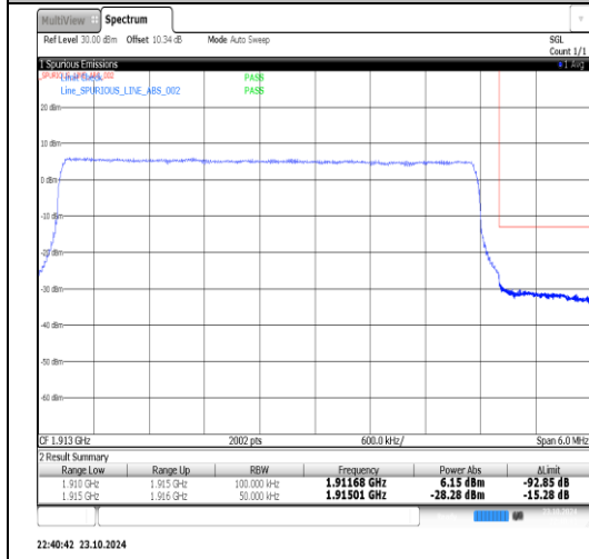
Band25-5MHz-16QAM-26065-1RB#0-PASS
