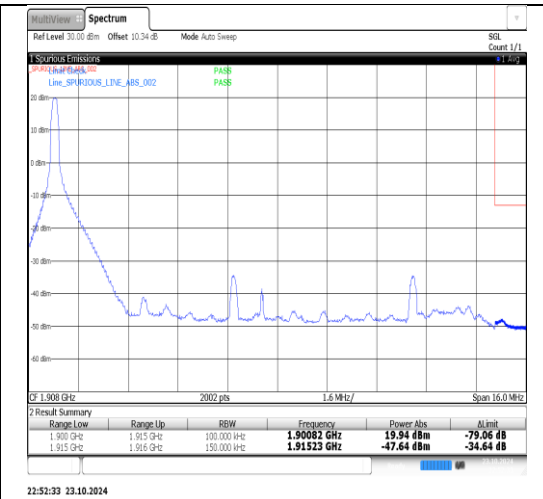
Band25-15MHz-QPSK-26615-1RB#74-PASS
