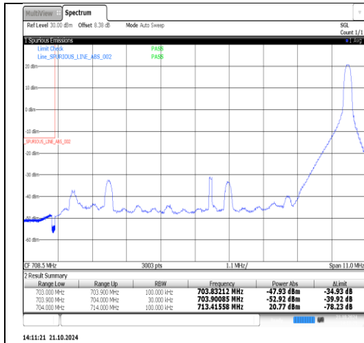
Band17-10MHz-QPSK-23800-50RB#0-PASS
