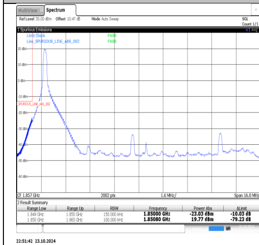
Band25-15MHz-16QAM-26115-1RB#74-PASS
