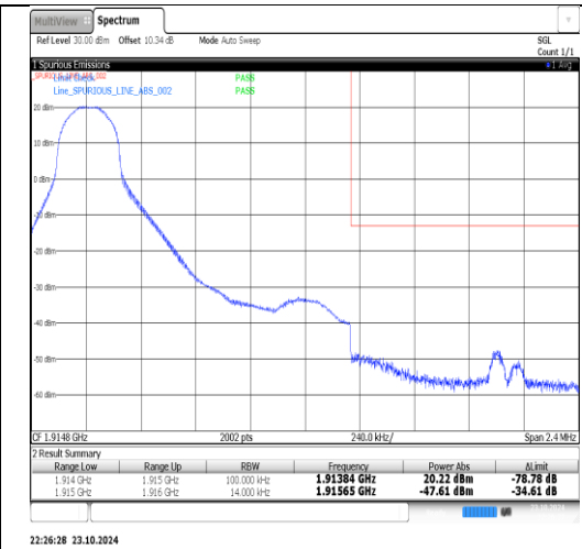
Band25-1.4MHz-QPSK-26683-1RB#5-PASS
