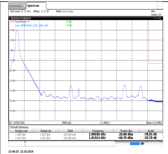
Band25-10MHz-QPSK-26640-1RB#49-PASS
