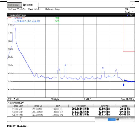
Band17-10MHz-16QAM-23800-1RB#49-PASS
