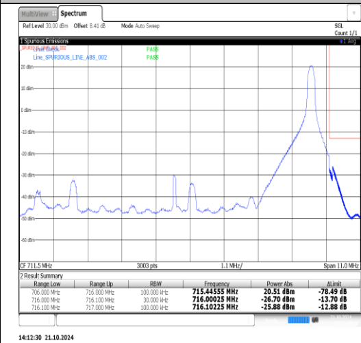
Band17-10MHz-16QAM-23780-50RB#0-PASS
