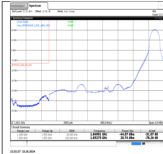
Band25-3MHz-QPSK-26675-15RB#0-PASS
