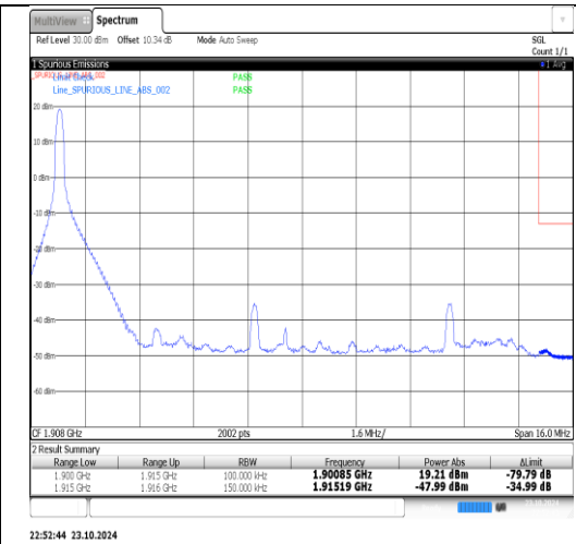
Band25-15MHz-16QAM-26615-1RB#74-PASS
