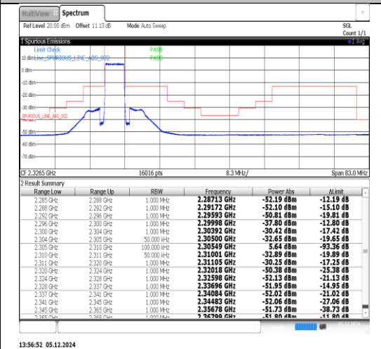
Band30-5MHz-QPSK-27735-1RB#0-PASS
