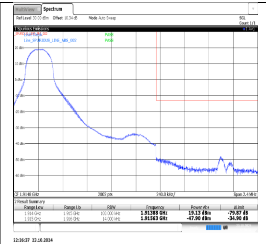
Band25-1.4MHz-16QAM-26683-1RB#5-PASS
