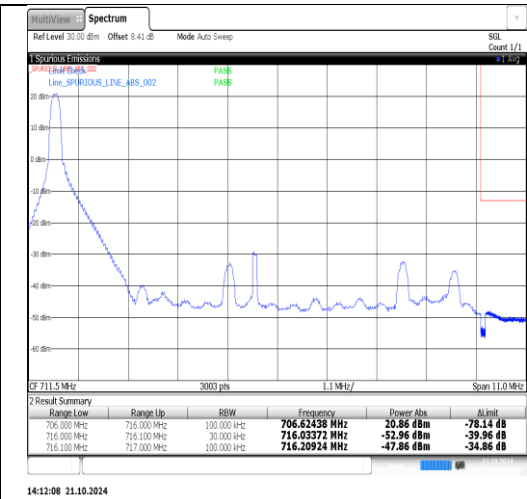
Band17-10MHz-QPSK-23800-1RB#49-PASS
