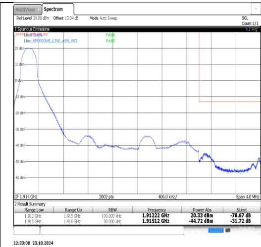
Band25-3MHz-QPSK-26675-1RB#14-PASS
