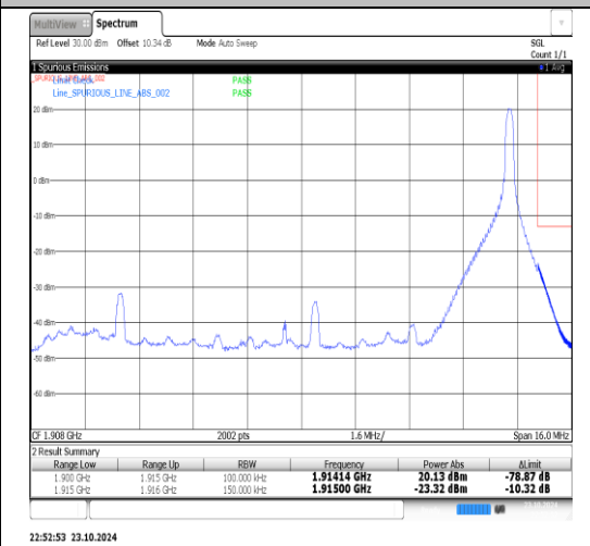
Band25-15MHz-16QAM-26115-75RB#0-PASS
