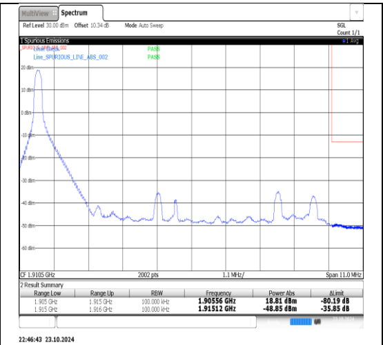
Band25-10MHz-16QAM-26640-1RB#49-PASS
