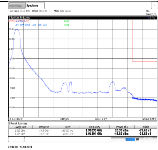
Band25-5MHz-QPSK-26665-1RB#24-PASS
