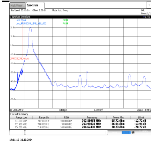
Band17-10MHz-16QAM-23780-1RB#49-PASS
