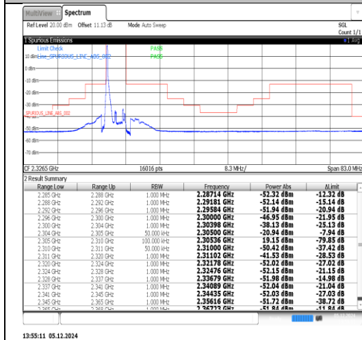
Band30-5MHz-QPSK-27685-1RB#24-PASS
