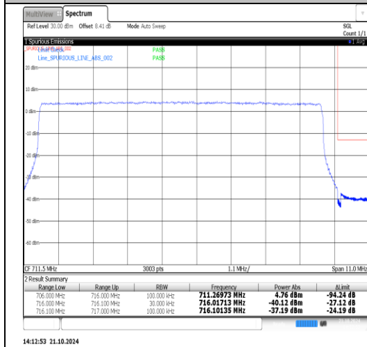
Band17-10MHz-16QAM-23780-1RB#0-PASS
