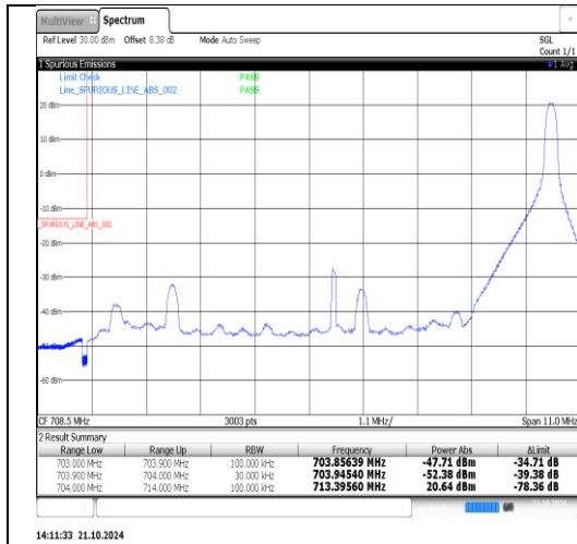
Band17-10MHz-16QAM-23800-50RB#0-PASS
