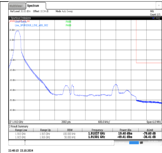
Band25-5MHz-16QAM-26665-1RB#24-PASS
