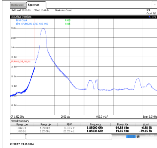
Band25-5MHz-16QAM-26065-1RB#24-PASS
