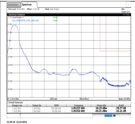
Band25-3MHz-16QAM-26675-1RB#14-PASS
