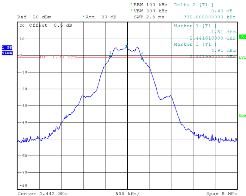
6 dB Bandwidth Plot on channel 20
