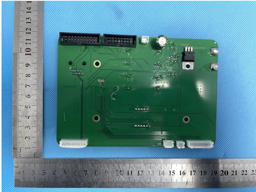
INTERNAL VIEW OF EUT CONTROL PANEL (FIGURE 2)
