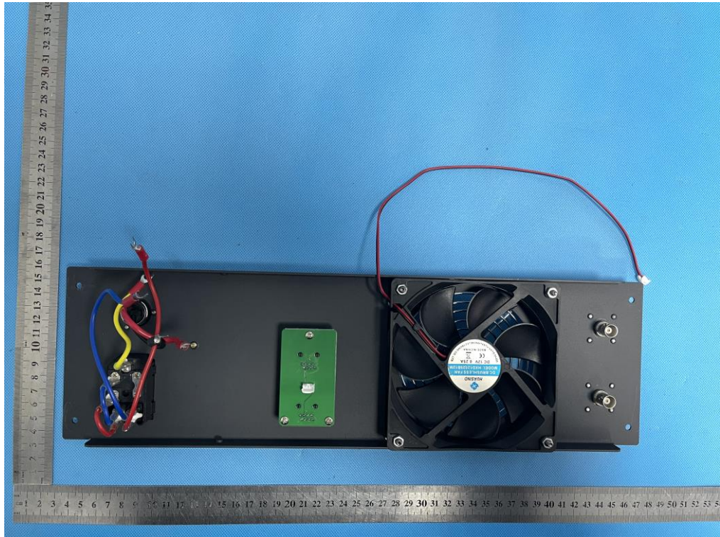
INTERNAL VIEW OF NETWORK WRITING PORT (FIGURE 1)
