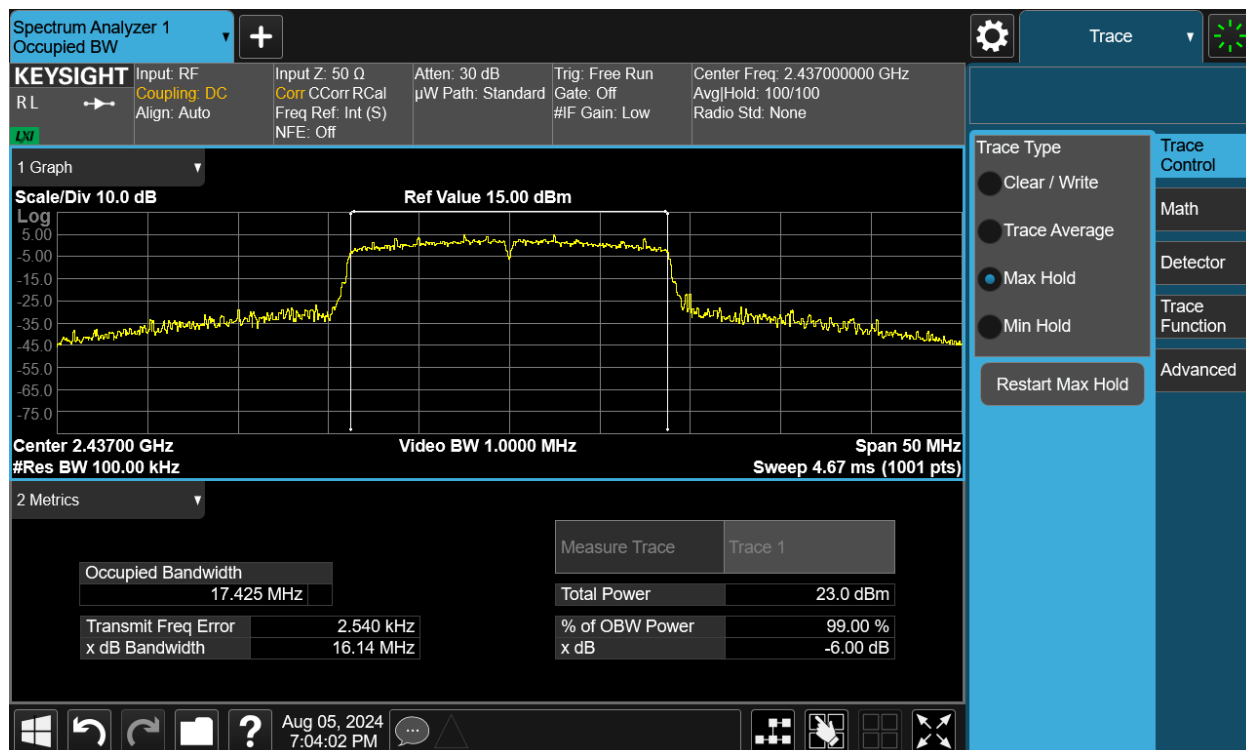
Plot 7-44. 6dB Bandwidth Plot MIMO ANT2 (802.11n (2.4GHz) – Ch. 6)
