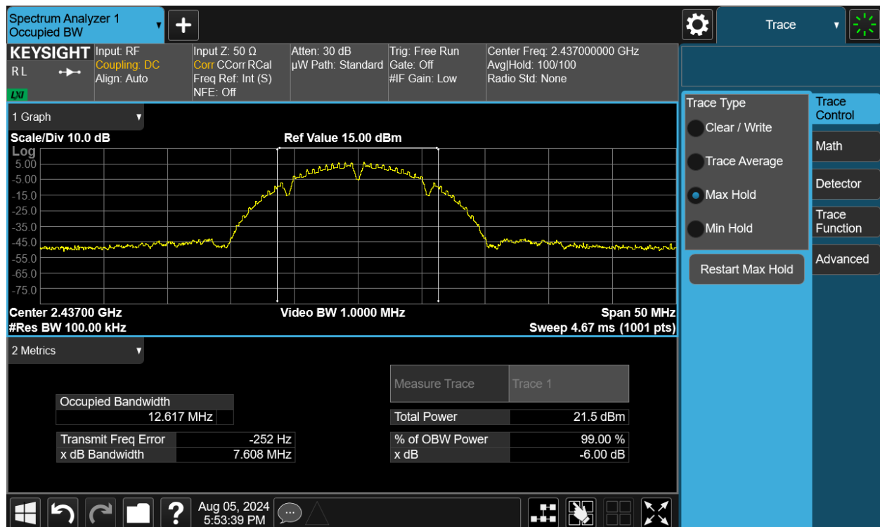
Plot 7-26. 6dB Bandwidth Plot MIMO ANT1 (802.11b – Ch. 6)
