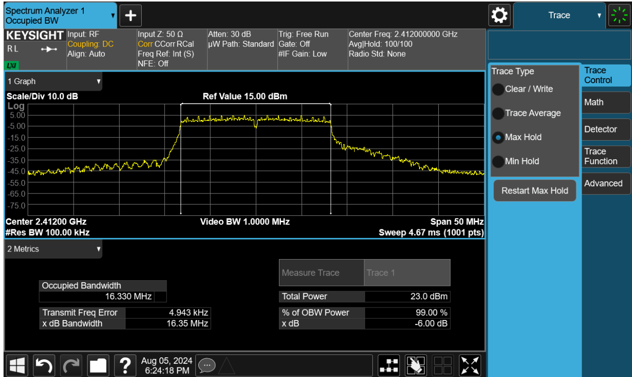
Plot 7-40. 6dB Bandwidth Plot MIMO ANT2 (802.11g – Ch. 1)
