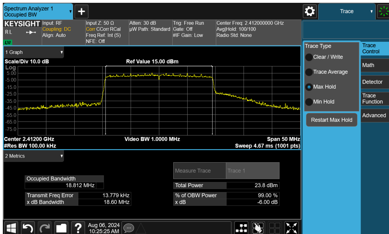
Plot 7-46. 6dB Bandwidth Plot MIMO ANT2 (802.11be (2.4GHz) – Ch. 1)
