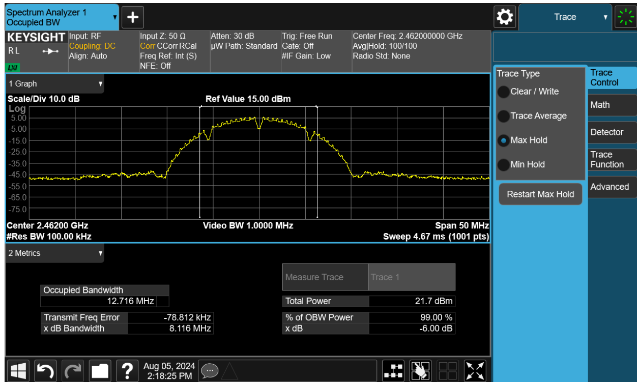
Plot 7-15. 6dB Bandwidth Plot SISO ANT2 (802.11b – Ch. 11)
