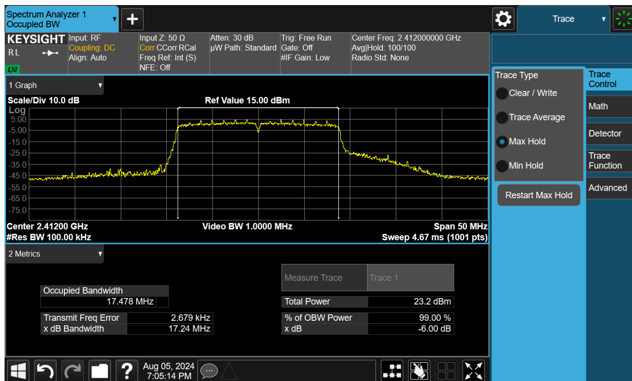
Plot 7-43. 6dB Bandwidth Plot MIMO ANT2 (802.11n (2.4GHz) – Ch. 1)
