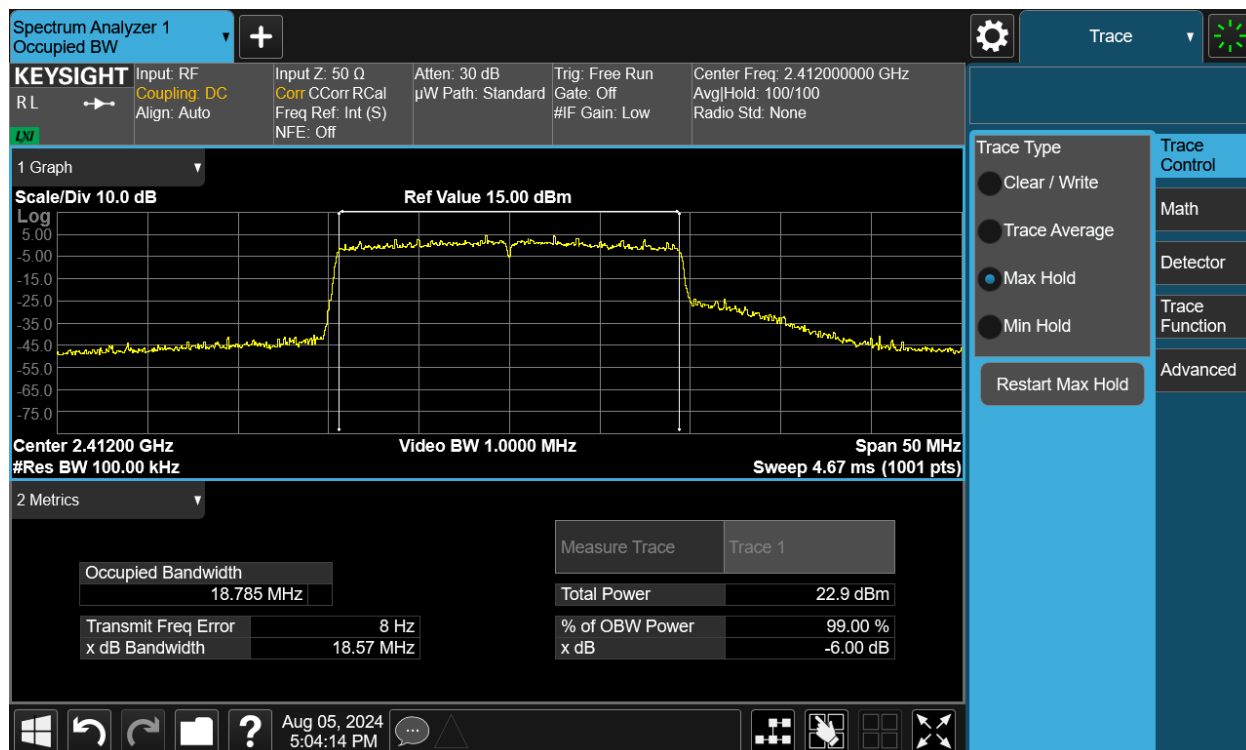
Plot 7-10. 6dB Bandwidth Plot SISO ANT1 (802.11be (2.4GHz) – Ch. 1)
