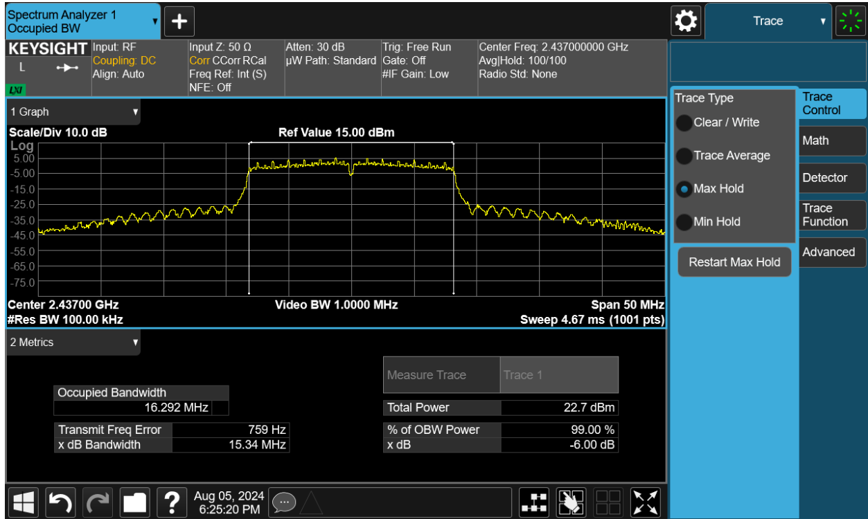
Plot 7-41. 6dB Bandwidth Plot MIMO ANT2 (802.11g – Ch. 6)
