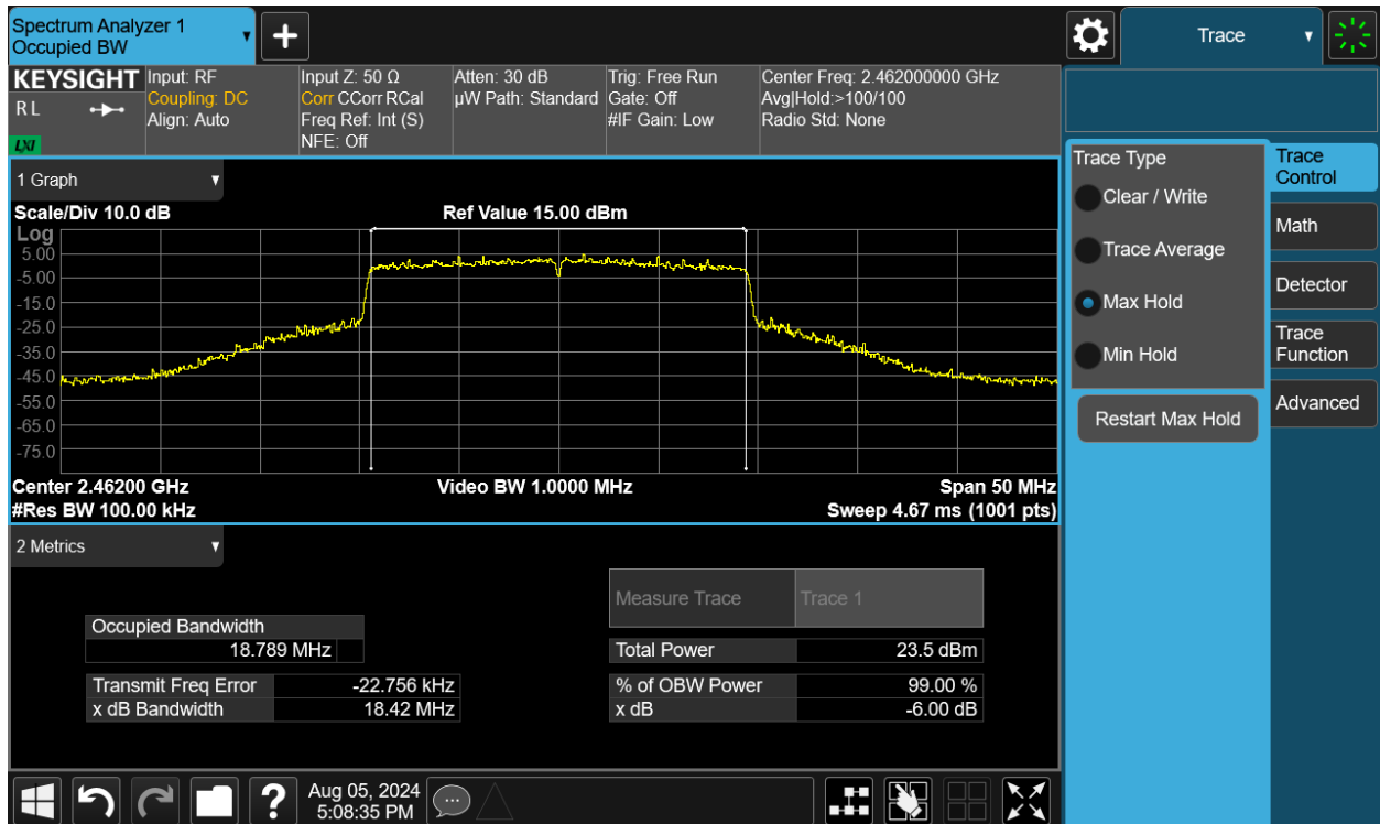
Plot 7-12. 6dB Bandwidth Plot SISO ANT1 (802.11be (2.4GHz) – Ch. 11)
