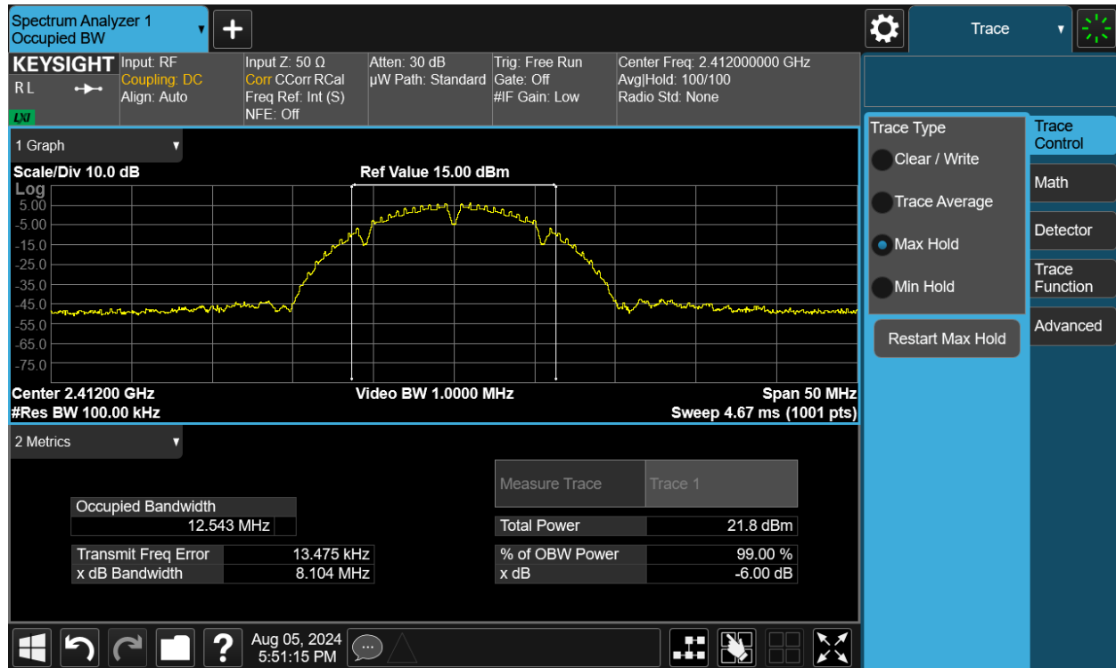
Plot 7-25. 6dB Bandwidth Plot MIMO ANT1 (802.11b – Ch. 1)
