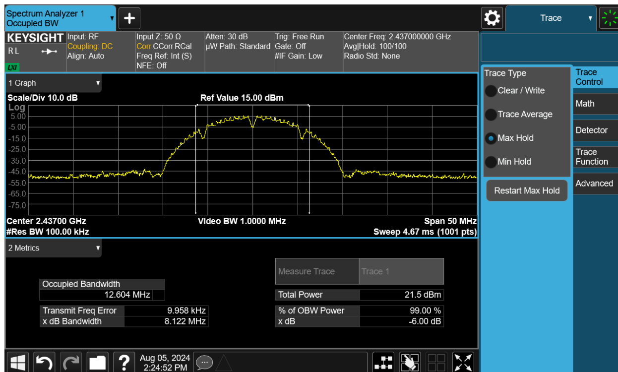
Plot 7-14. 6dB Bandwidth Plot SISO ANT2 (802.11b – Ch. 6)
