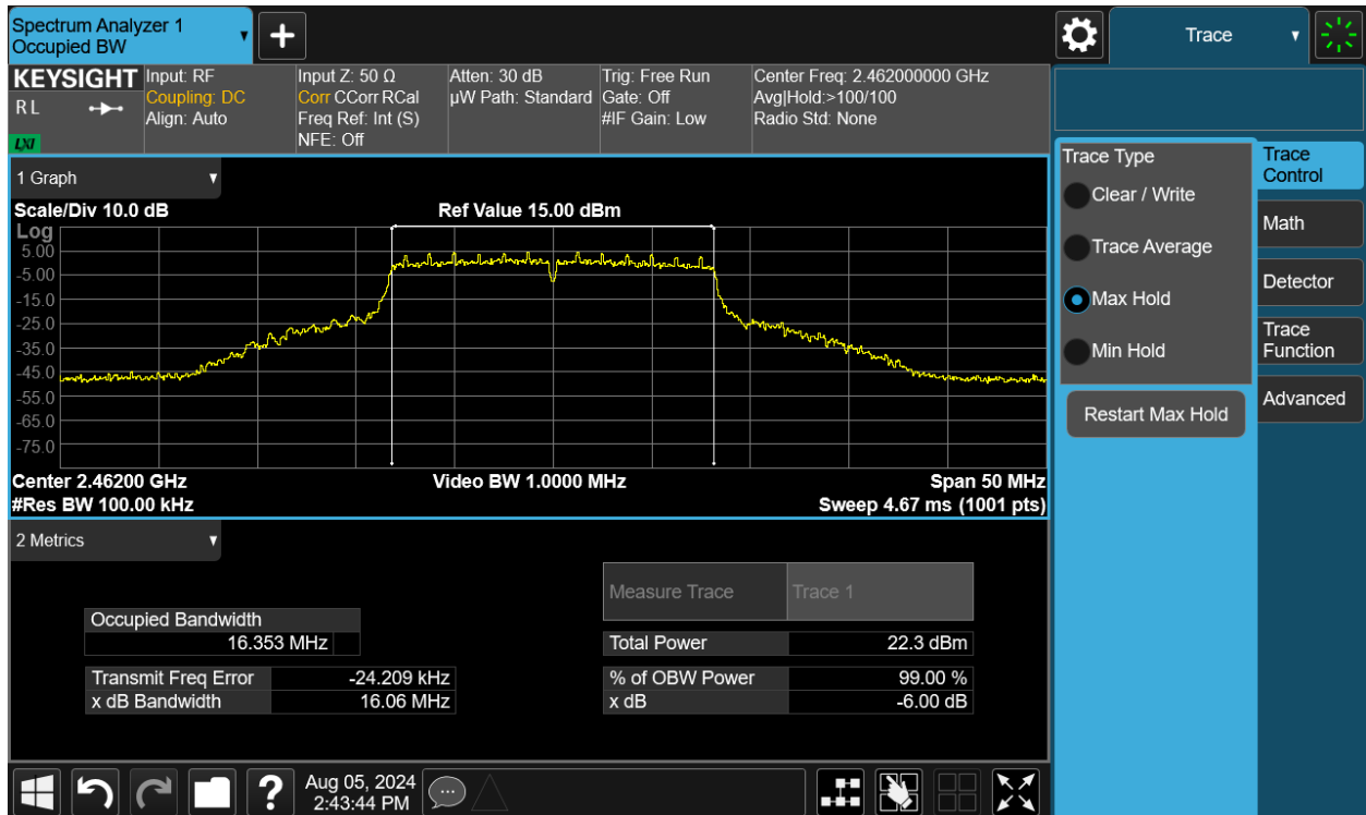
Plot 7-18. 6dB Bandwidth Plot SISO ANT2 (802.11g – Ch. 11)
