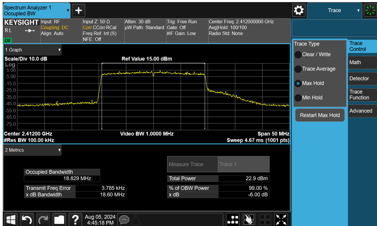
Plot 7-22. 6dB Bandwidth Plot SISO ANT2 (802.11be (2.4GHz) – Ch. 1)
