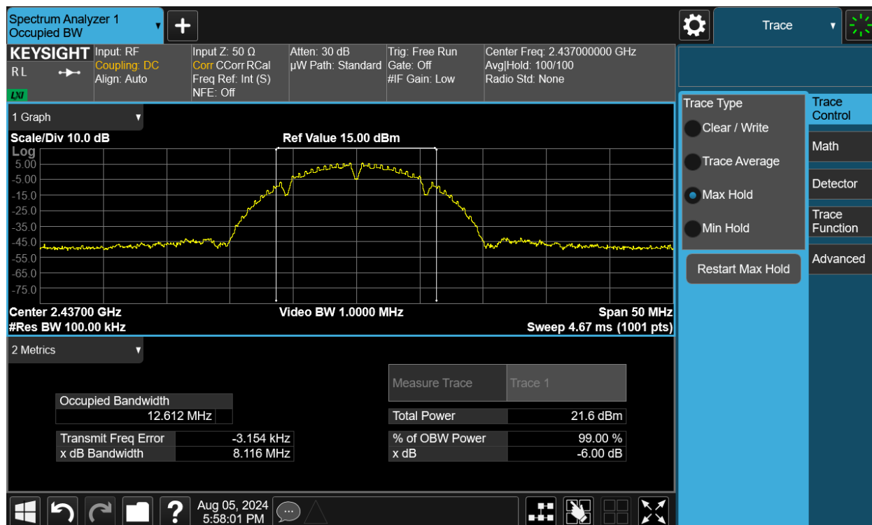
Plot 7-38. 6dB Bandwidth Plot MIMO ANT2 (802.11b – Ch. 6)
