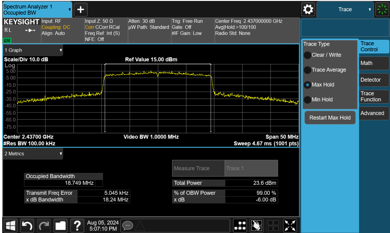
Plot 7-11. 6dB Bandwidth Plot SISO ANT1 (802.11be (2.4GHz) – Ch. 6)
