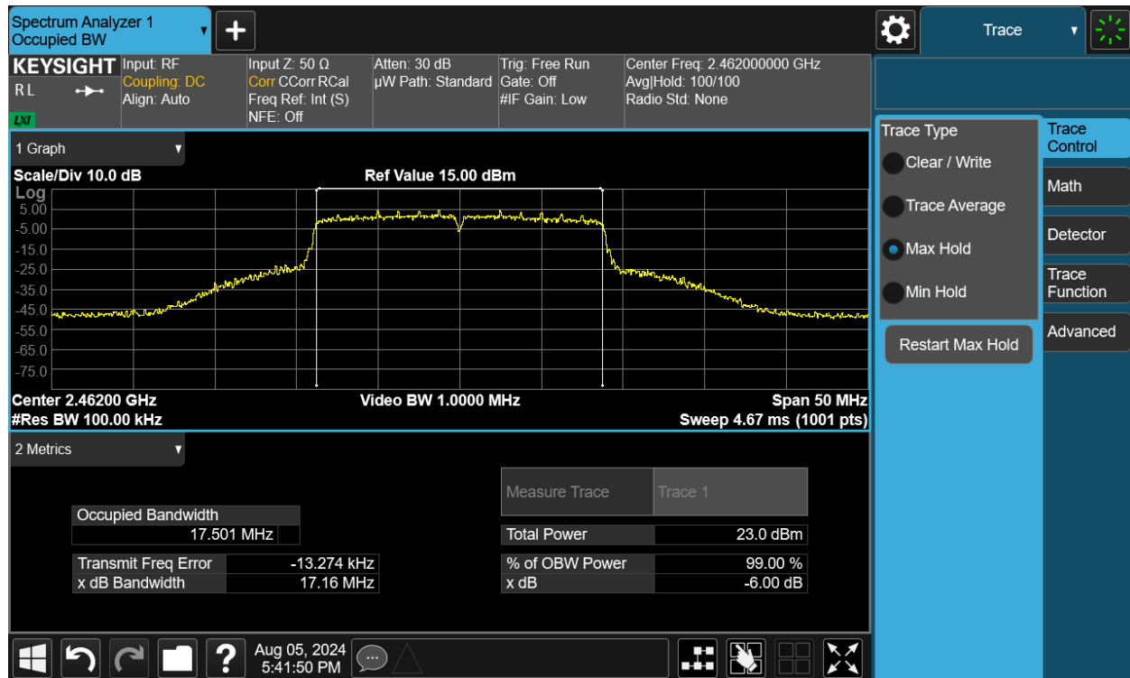
Plot 7-21. 6dB Bandwidth Plot SISO ANT2 (802.11n (2.4GHz) – Ch. 11)
