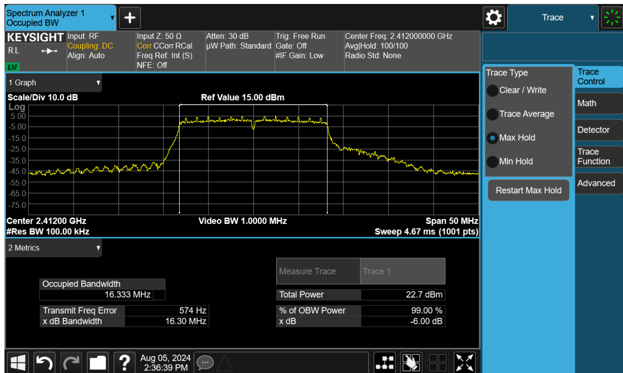
Plot 7-16. 6dB Bandwidth Plot SISO ANT2 (802.11g – Ch. 1)
