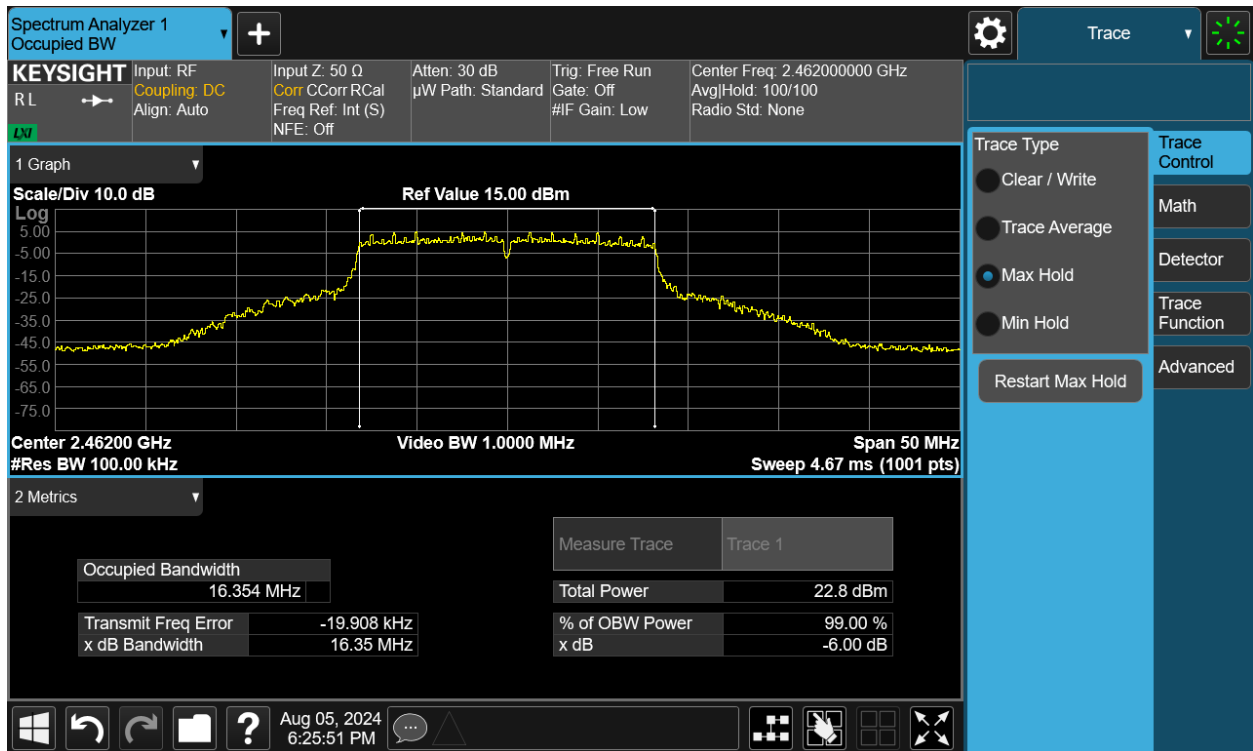
Plot 7-42. 6dB Bandwidth Plot MIMO ANT2 (802.11g – Ch. 11)
