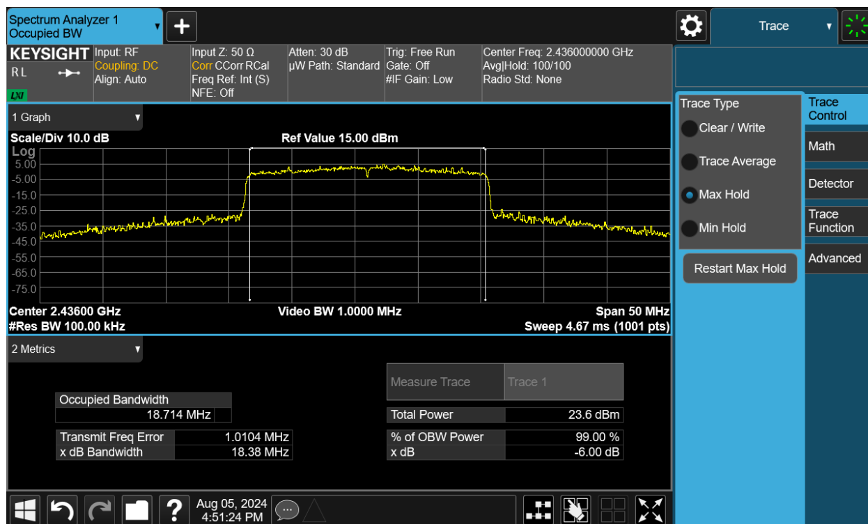
Plot 7-23. 6dB Bandwidth Plot SISO ANT2 (802.11be (2.4GHz) – Ch. 6)
