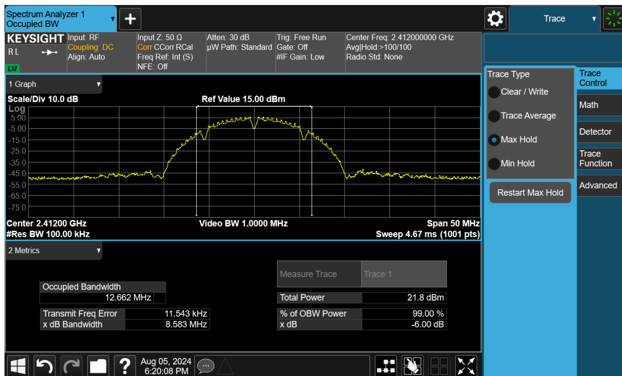
Plot 7-37. 6dB Bandwidth Plot MIMO ANT2 (802.11b – Ch. 1)
