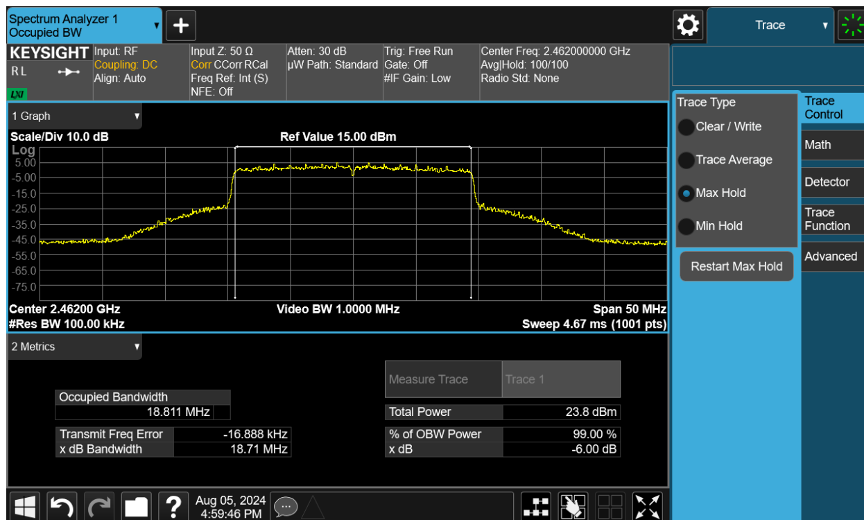
Plot 7-24. 6dB Bandwidth Plot SISO ANT2 (802.11be (2.4GHz) – Ch. 11)
