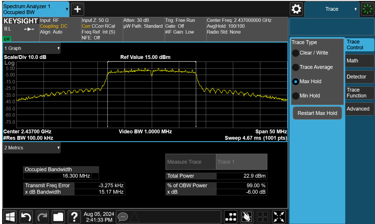
Plot 7-17. 6dB Bandwidth Plot SISO ANT2 (802.11g – Ch. 6)
