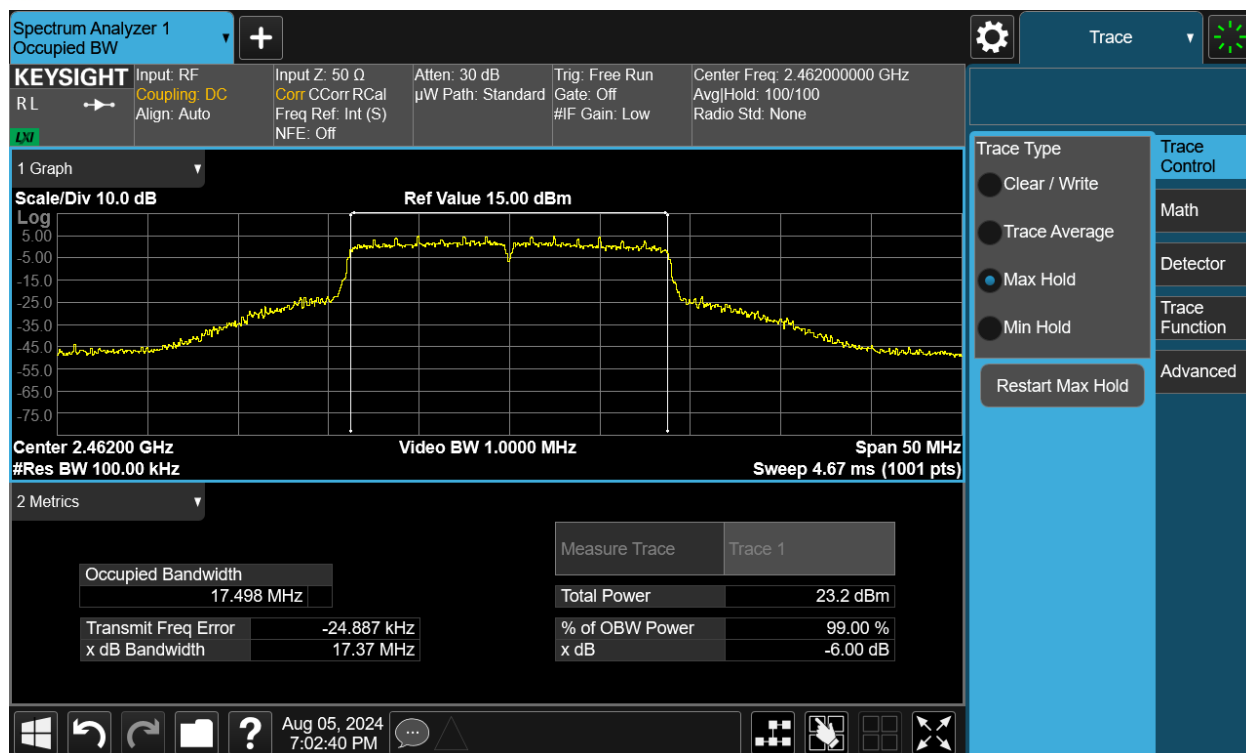
Plot 7-45. 6dB Bandwidth Plot MIMO ANT2 (802.11n (2.4GHz) – Ch. 11)
