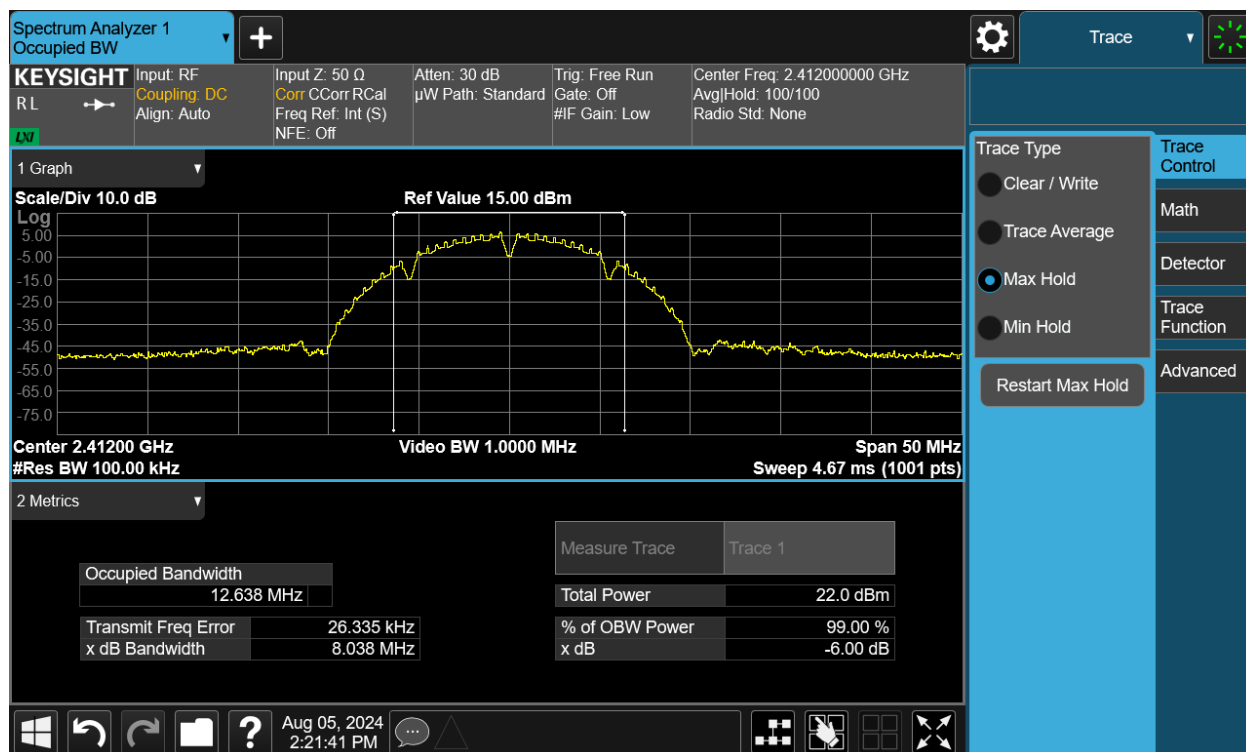
Plot 7-13. 6dB Bandwidth Plot SISO ANT2 (802.11b – Ch. 1)
