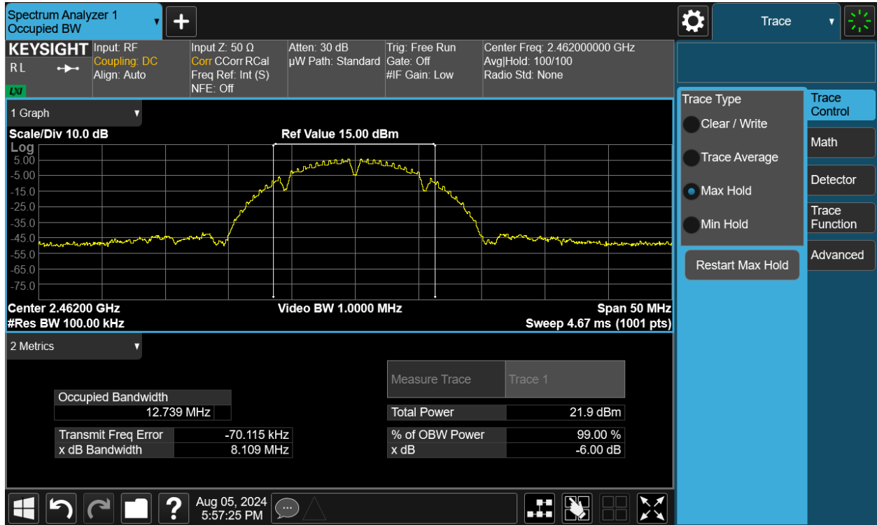
Plot 7-39. 6dB Bandwidth Plot MIMO ANT2 (802.11b – Ch. 11)
