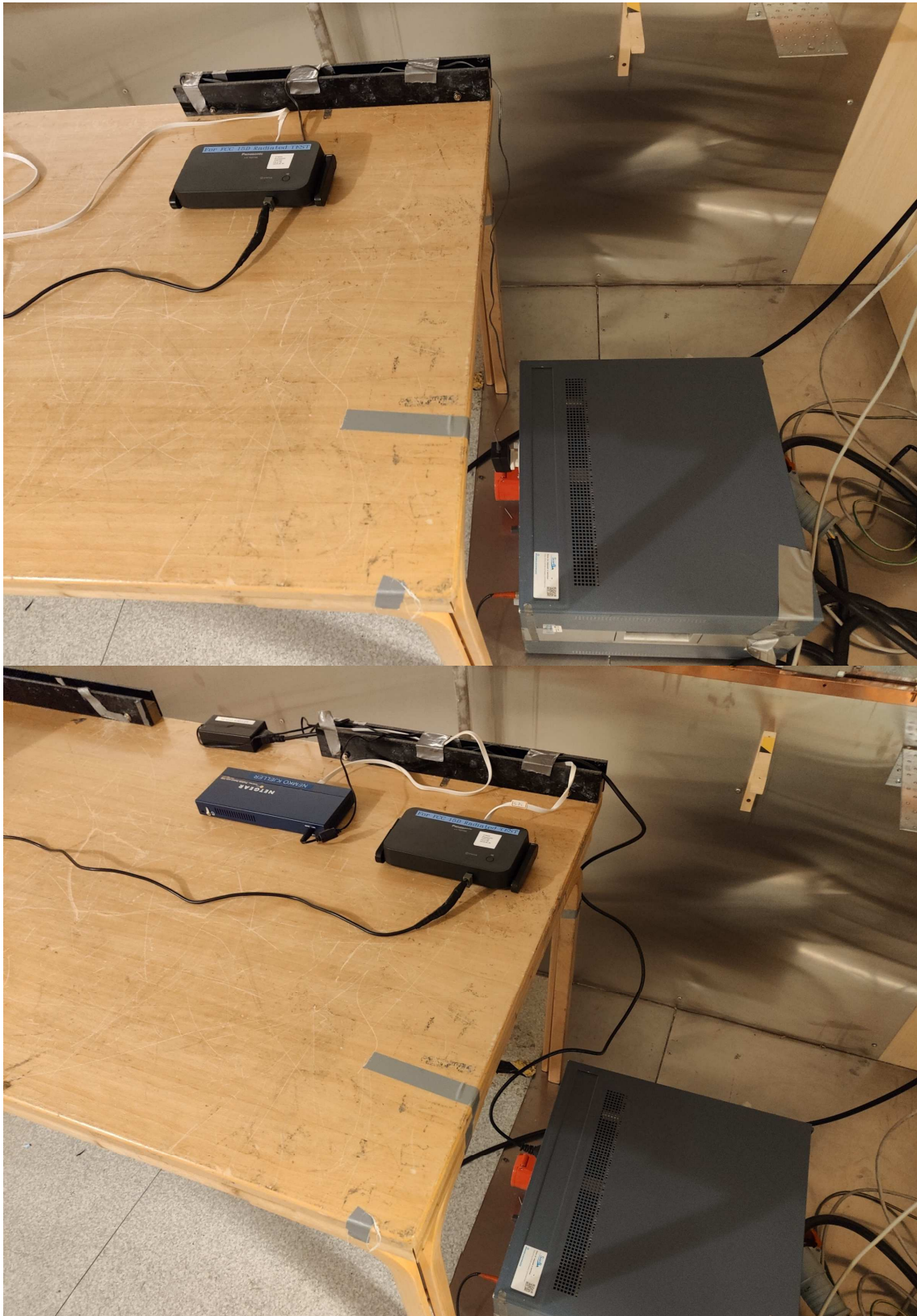
Power-line Conducted Emissions Test
