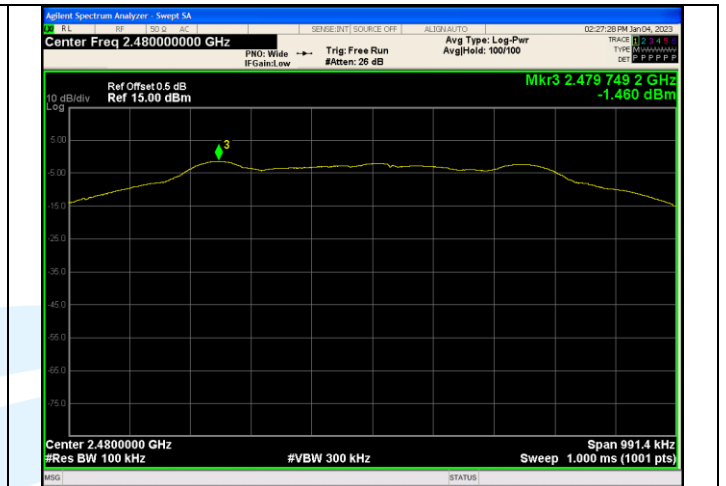
In-Band Reference Level LE_Channel 39
