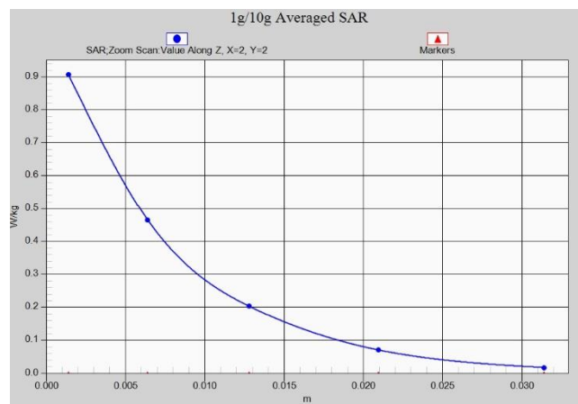
Fig. 1-41 Z-Scan at power reference point (wifi2450)
