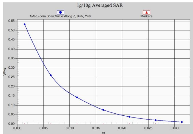
Fig. 1-55 Z-Scan at power reference point (n41)
