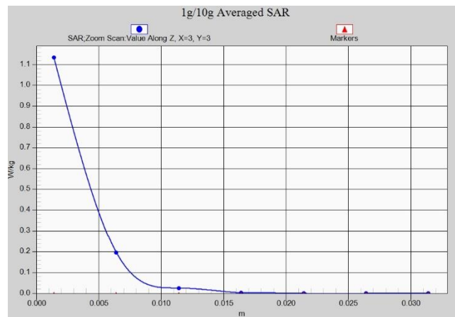
Fig. 1-43 Z-Scan at power reference point (wifi5G)
