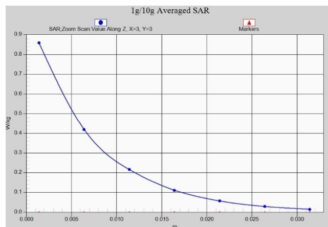
Fig. 1-30 Z-Scan at power reference point (LTE Band38)
