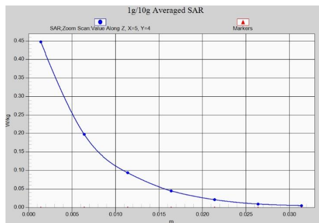
Fig. 1-54 Z-Scan at power reference point (n41)
