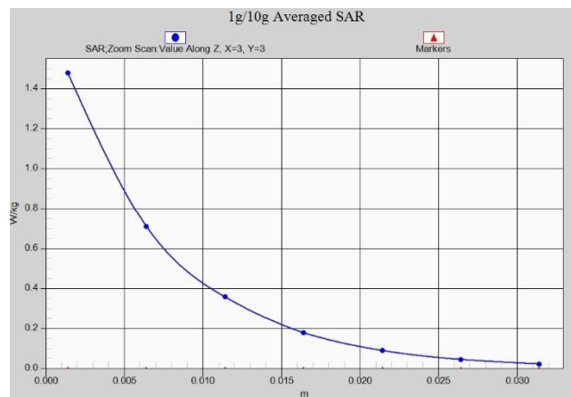
Fig. 1-34 Z-Scan at power reference point (LTE Band41)
