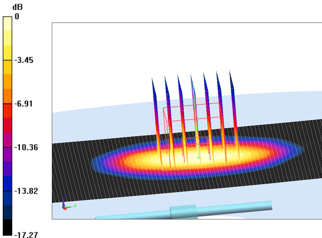
Fig.B.9 validation 1900 MHz 250mW
