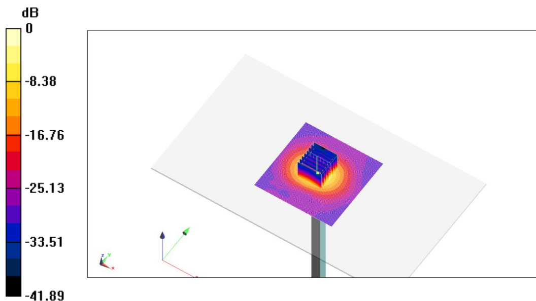
Fig.B.16 validation 5600 MHz 100mW
