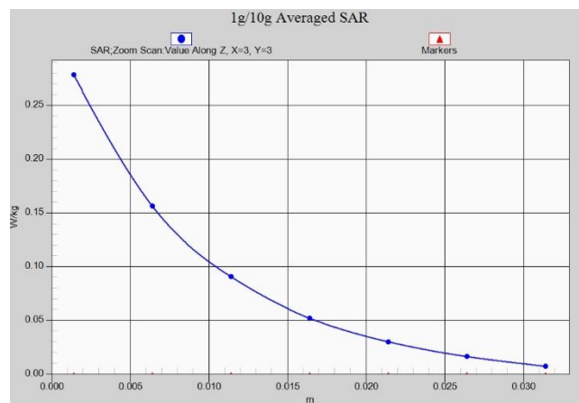
Fig. 1-50 Z-Scan at power reference point (n41)
