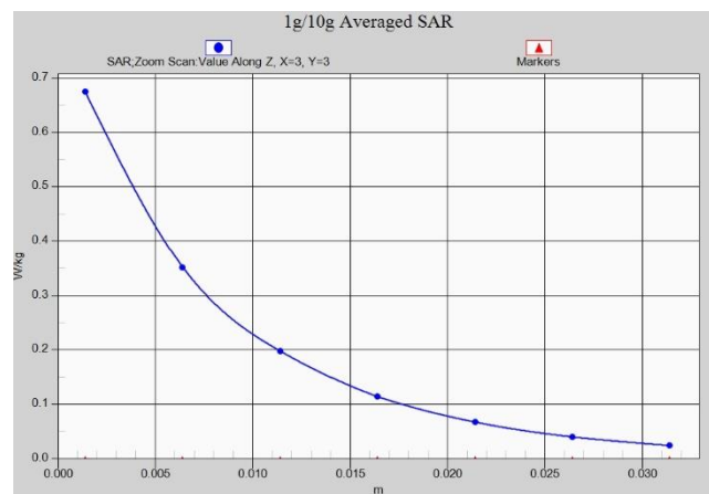
Fig. 1-59 Z-Scan at power reference point (n66)
