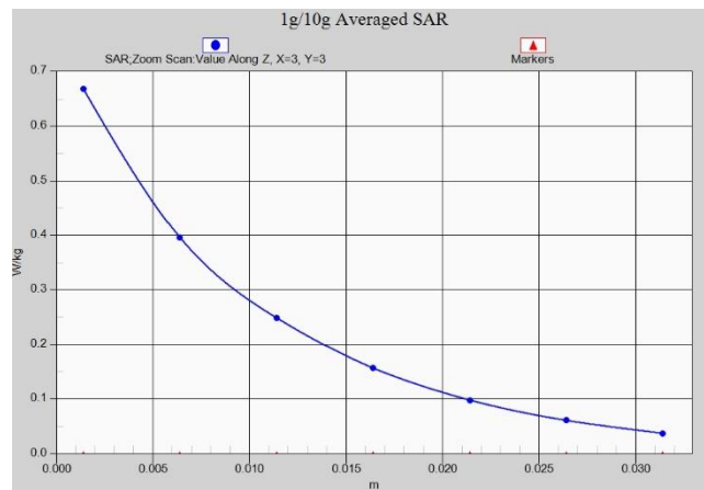
Fig. 1-46 Z-Scan at power reference point (n25)
