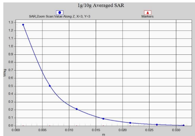
Fig. 1-40 Z-Scan at power reference point (wifi2450)
