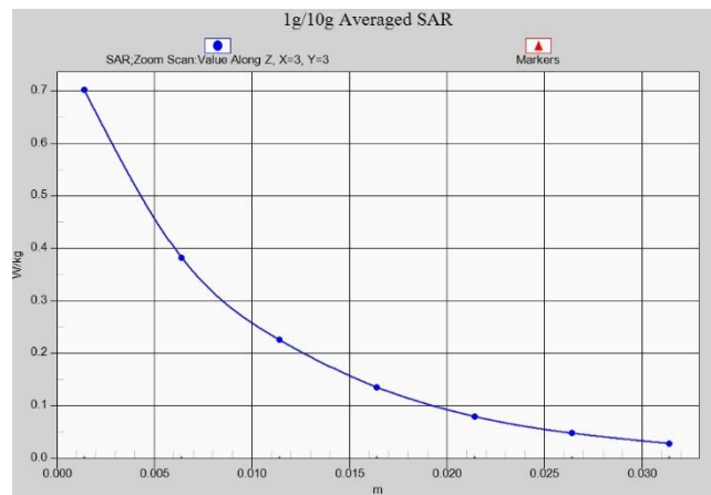
Fig. 1-61 Z-Scan at power reference point (n66)
