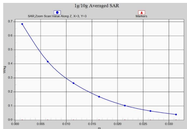
Fig. 1-45 Z-Scan at power reference point (n25)
