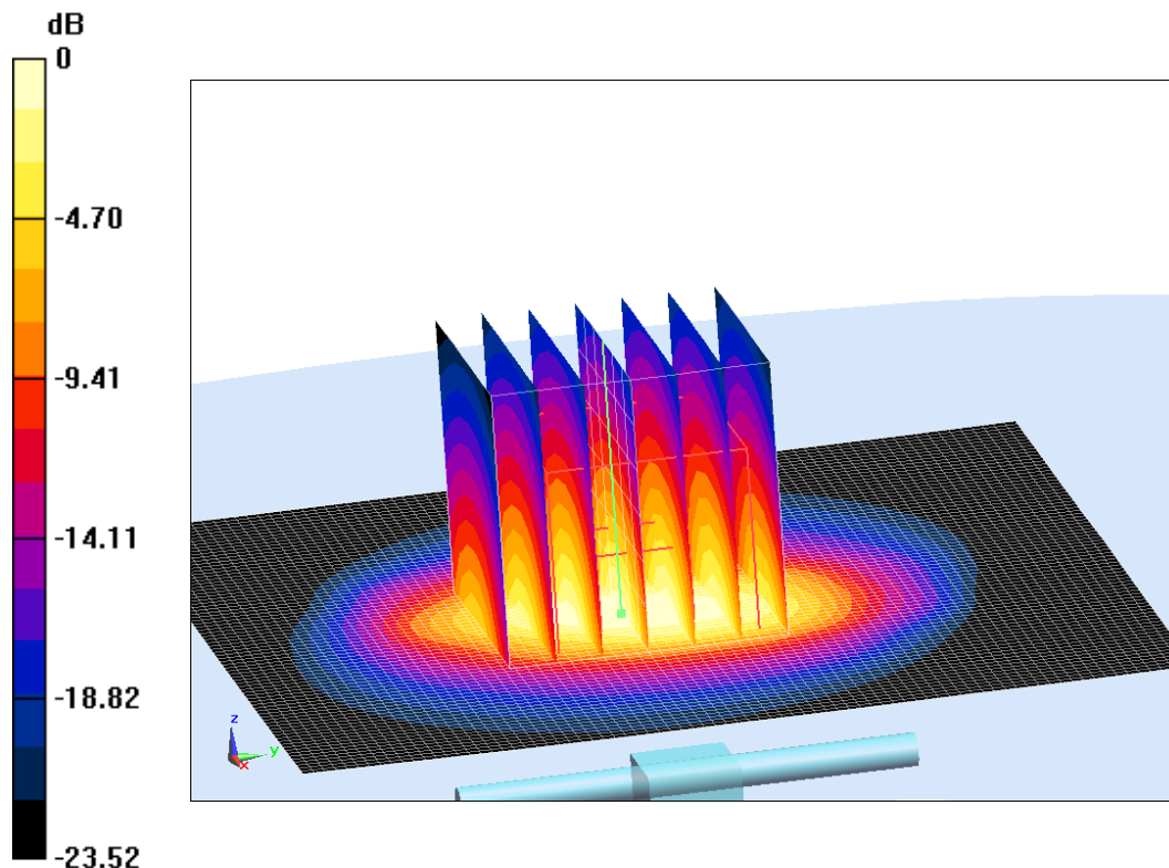
Fig.B.14 validation 2600 MHz 250mW
