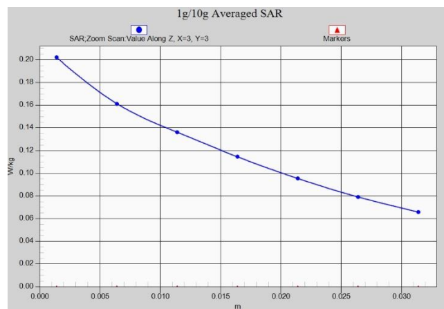
Fig. 1-62 Z-Scan at power reference point (n71)
