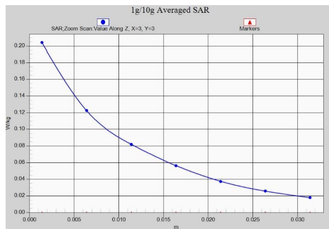
Fig. 1-44 Z-Scan at power reference point (n25)
