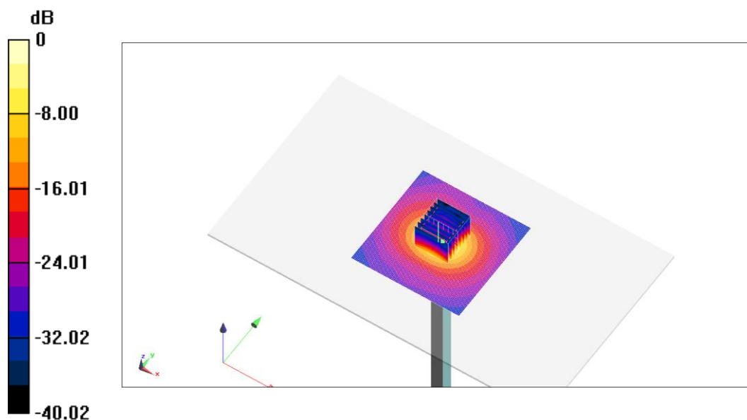
Fig.B.15 validation 5250 MHz 100mW
