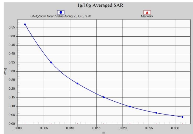
Fig. 1-58 Z-Scan at power reference point (n66)
