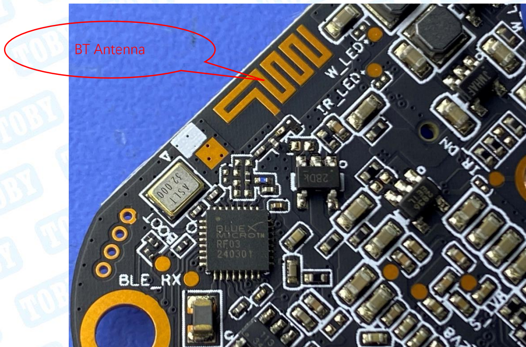
Photo 19 Appearance of PCB
