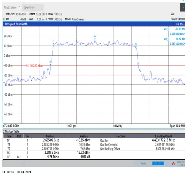
Band41-5MHz-64QAM-41565-25RB#0-PASS
