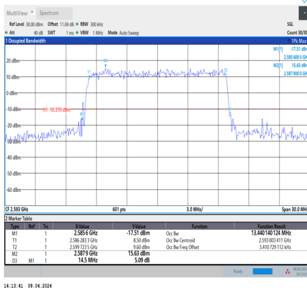
Band41-15MHz-16QAM-40620-75RB#0-PASS
