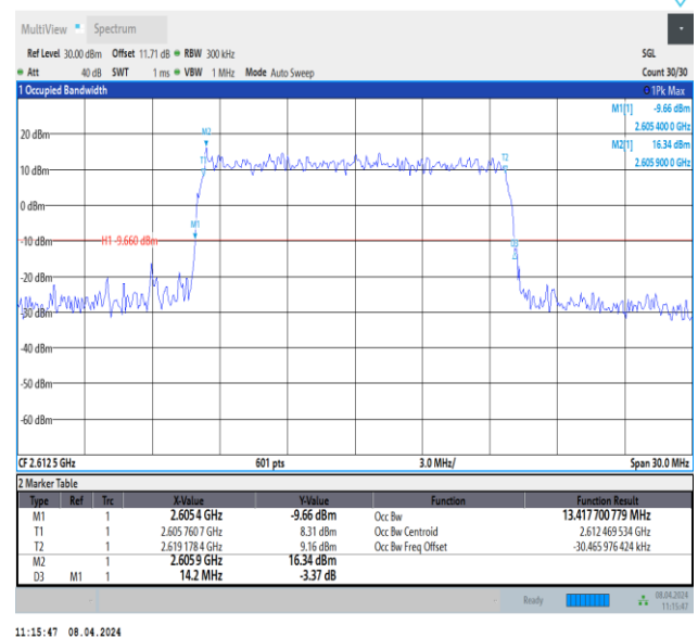
Band38-15MHz-16QAM-38175-75RB#0-PASS
