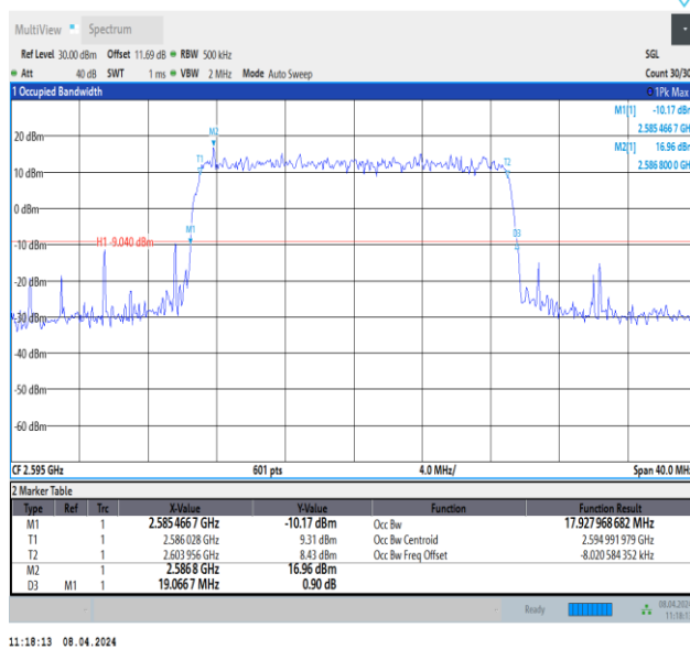
Band38-20MHz-64QAM-38000-100RB#0-PASS
