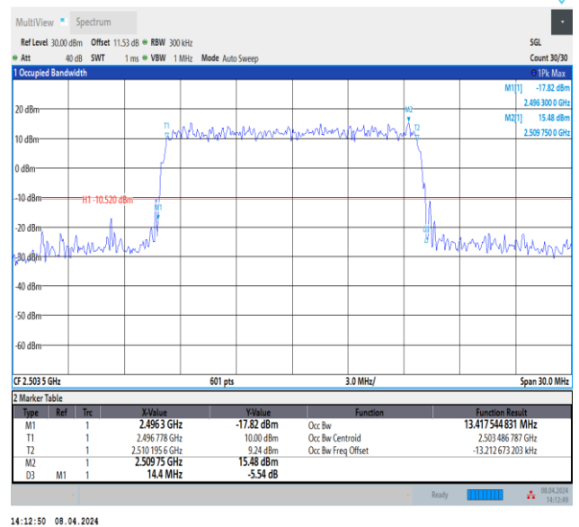
Band41-15MHz-16QAM-39725-75RB#0-PASS
