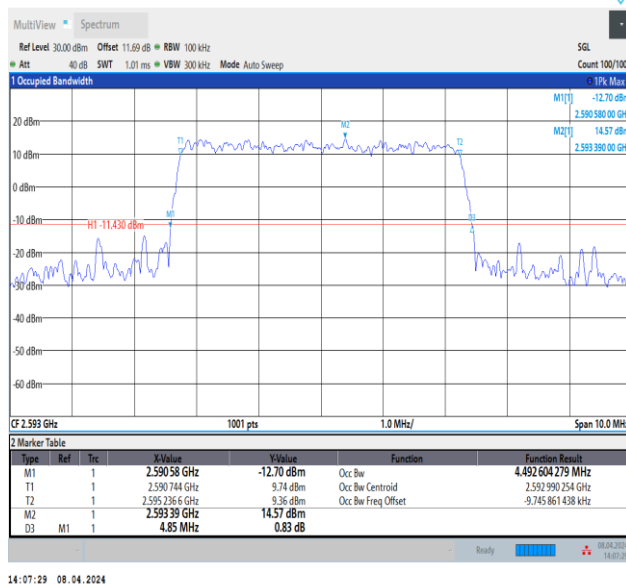
Band41-5MHz-16QAM-40620-25RB#0-PASS
