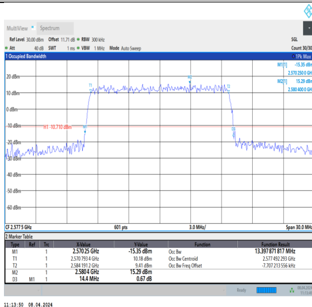
Band38-15MHz-QPSK-37825-75RB#0-PASS
