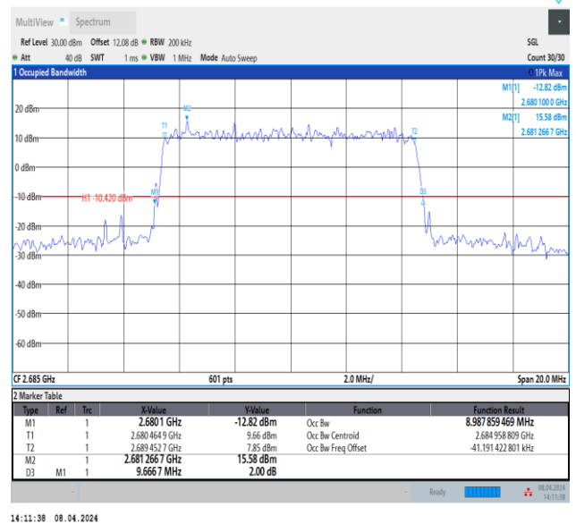
Band41-10MHz-64QAM-41540-50RB#0-PASS
