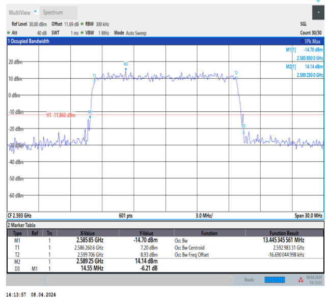
Band41-15MHz-64QAM-40620-75RB#0-PASS
