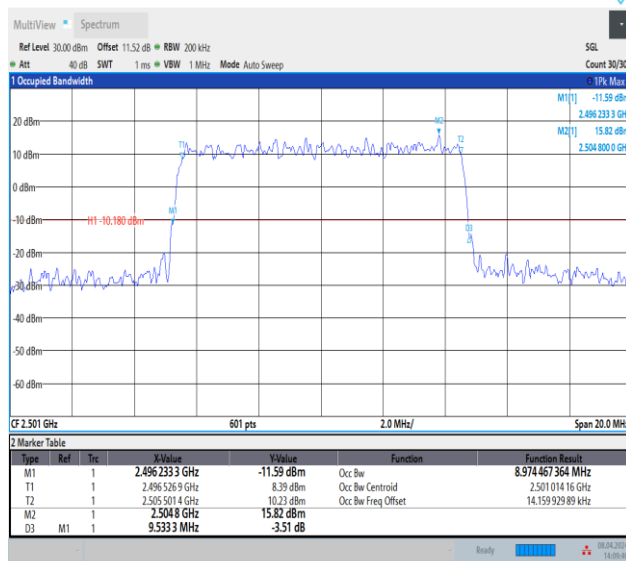
Band41-10MHz-16QAM-39700-50RB#0-PASS
