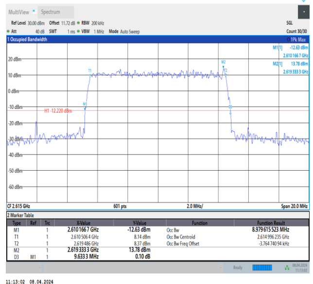
Band38-10MHz-64QAM-38200-50RB#0-PASS
