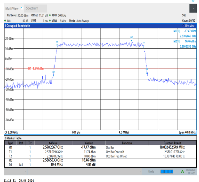
Band38-20MHz-QPSK-37850-100RB#0-PASS
