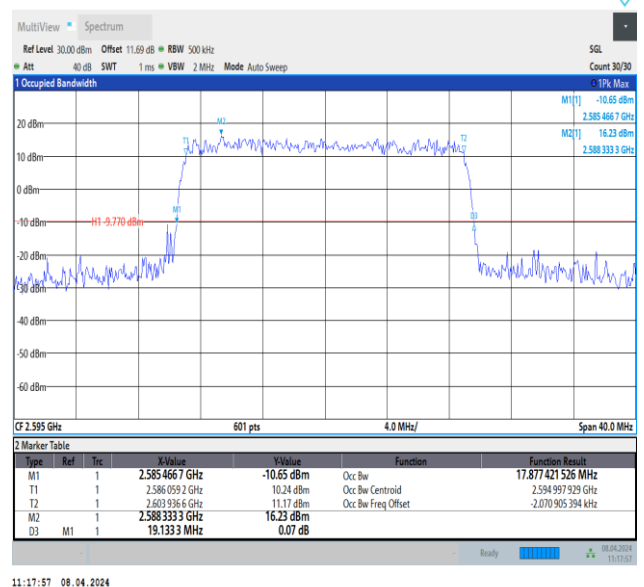
Band38-20MHz-16QAM-38000-100RB#0-PASS
