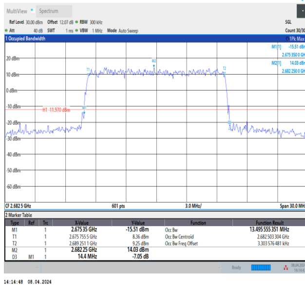
Band41-15MHz-64QAM-41515-75RB#0-PASS
