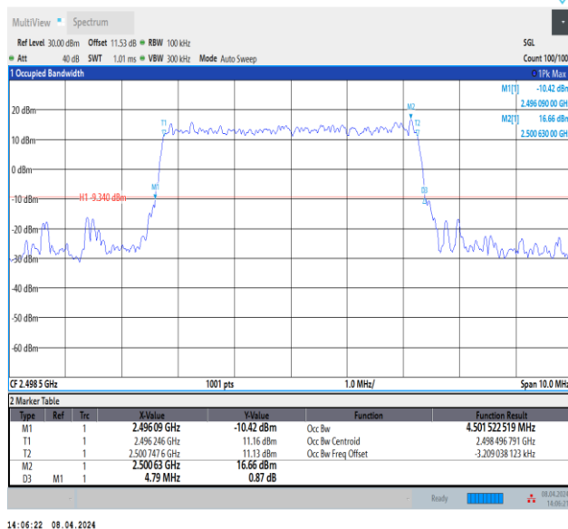
Band41-5MHz-QPSK-39675-25RB#0-PASS
