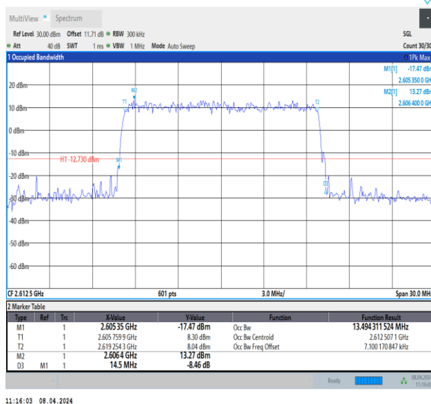
Band38-15MHz-64QAM-38175-75RB#0-PASS
