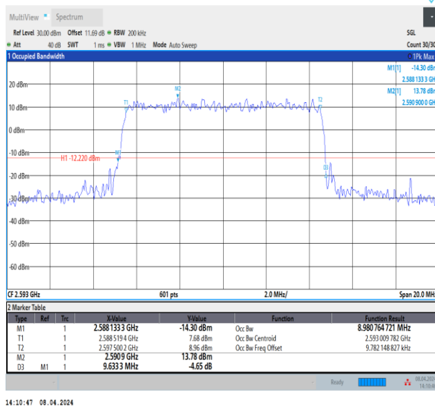
Band41-10MHz-64QAM-40620-50RB#0-PASS
