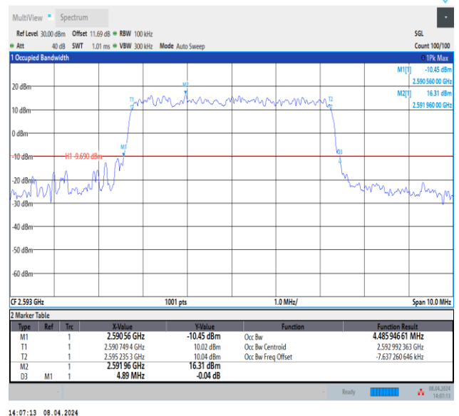
Band41-5MHz-QPSK-40620-25RB#0-PASS
