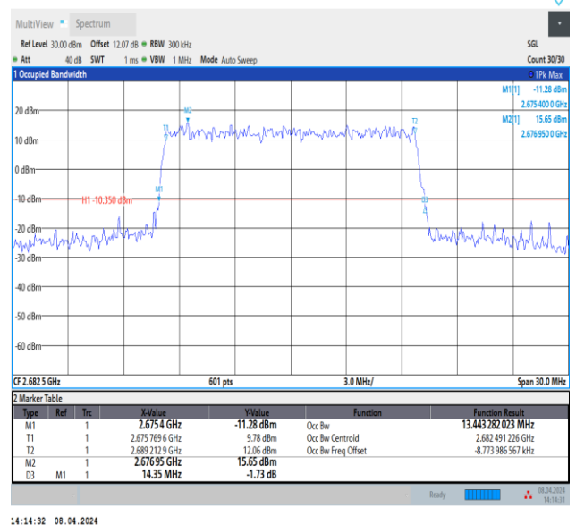
Band41-15MHz-16QAM-41515-75RB#0-PASS
