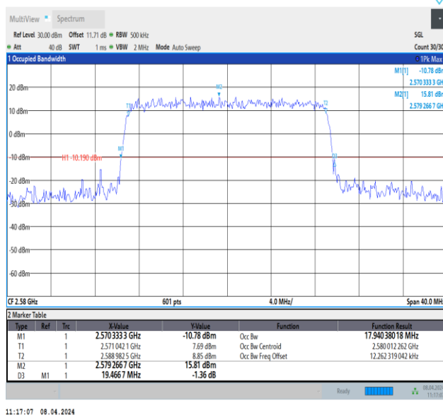
Band38-20MHz-16QAM-37850-100RB#0-PASS
