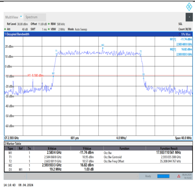
Band41-20MHz-16QAM-40620-100RB#0-PASS
