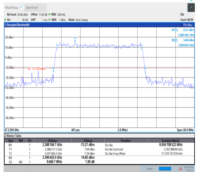
Band41-10MHz-16QAM-40620-50RB#0-PASS
