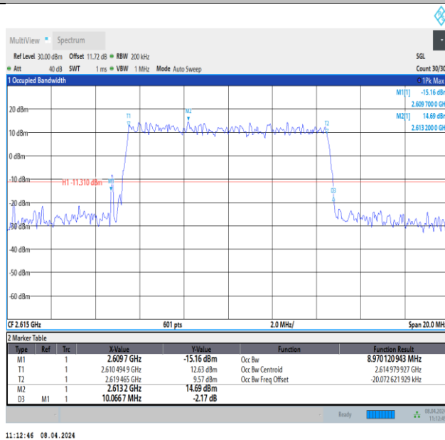
Band38-10MHz-16QAM-38200-50RB#0-PASS
