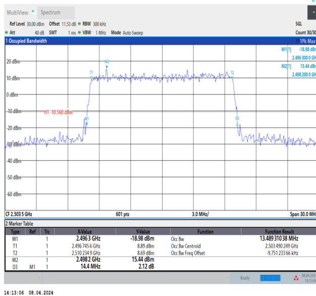
Band41-15MHz-64QAM-39725-75RB#0-PASS
