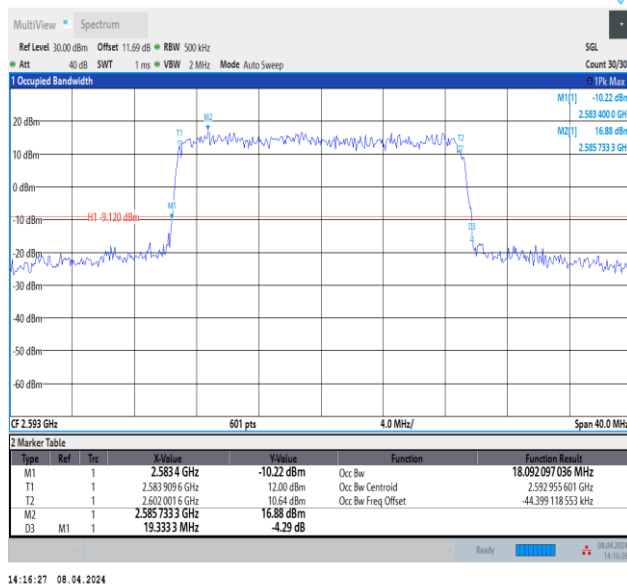
Band41-20MHz-QPSK-40620-100RB#0-PASS
