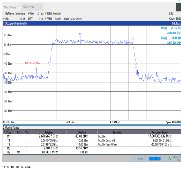
Band38-20MHz-16QAM-38150-100RB#0-PASS
