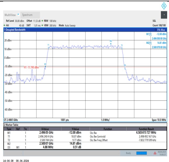
Band41-5MHz-16QAM-39675-25RB#0-PASS
