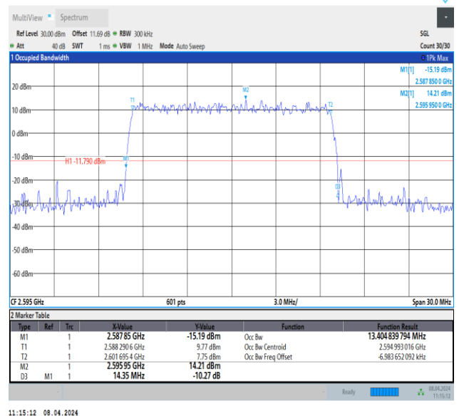
Band38-15MHz-64QAM-38000-75RB#0-PASS
