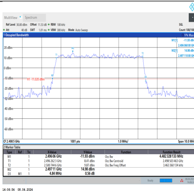
Band41-5MHz-64QAM-39675-25RB#0-PASS
