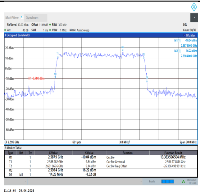
Band38-15MHz-QPSK-38000-75RB#0-PASS
