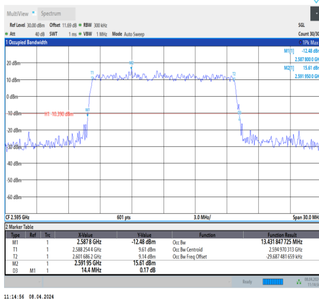
Band38-15MHz-16QAM-38000-75RB#0-PASS
