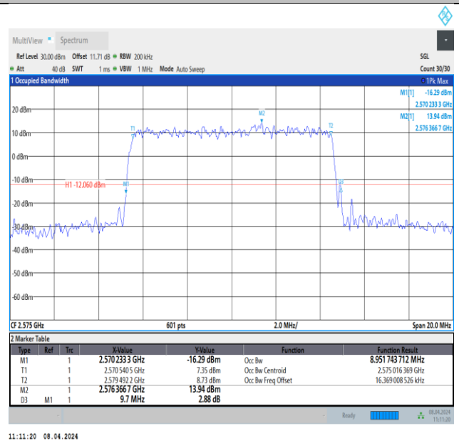
Band38-10MHz-64QAM-37800-50RB#0-PASS
