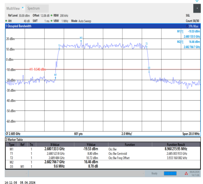
Band41-10MHz-QPSK-41540-50RB#0-PASS
