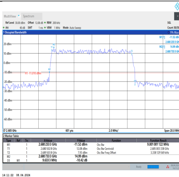
Band41-10MHz-16QAM-41540-50RB#0-PASS
