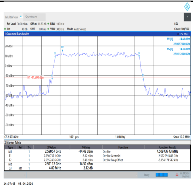
Band41-5MHz-64QAM-40620-25RB#0-PASS
