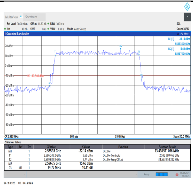
Band41-15MHz-QPSK-40620-75RB#0-PASS
