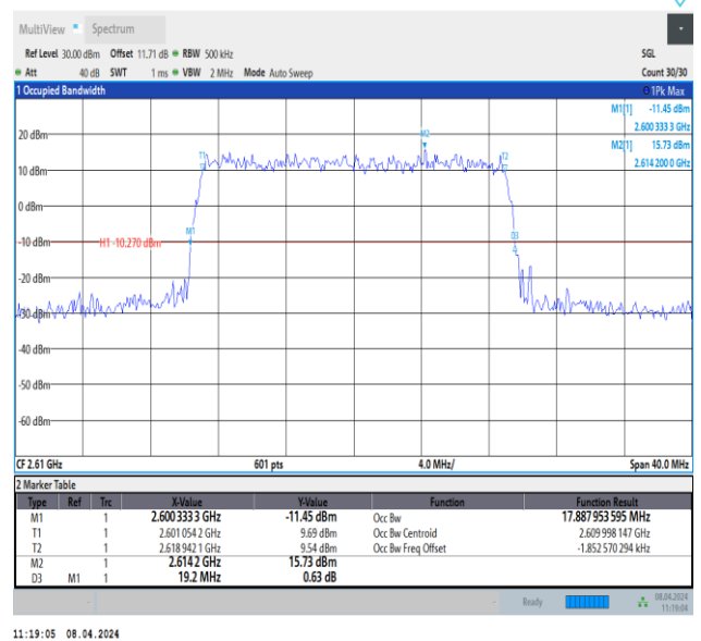
Band38-20MHz-64QAM-38150-100RB#0-PASS
