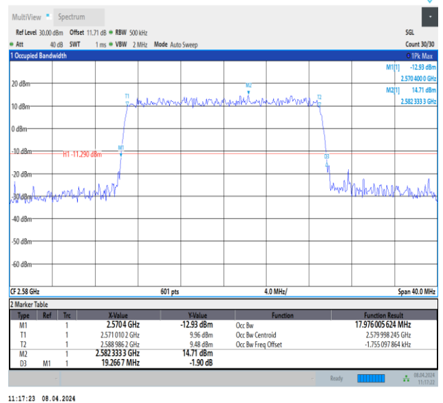
Band38-20MHz-64QAM-37850-100RB#0-PASS
