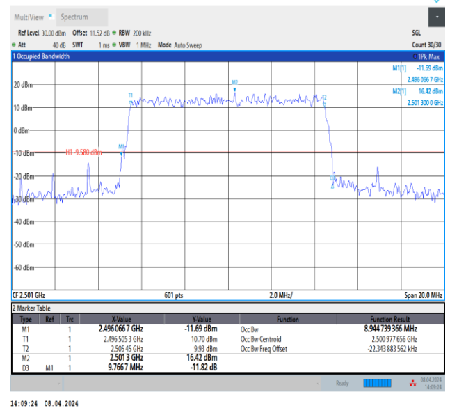
Band41-10MHz-QPSK-39700-50RB#0-PASS
