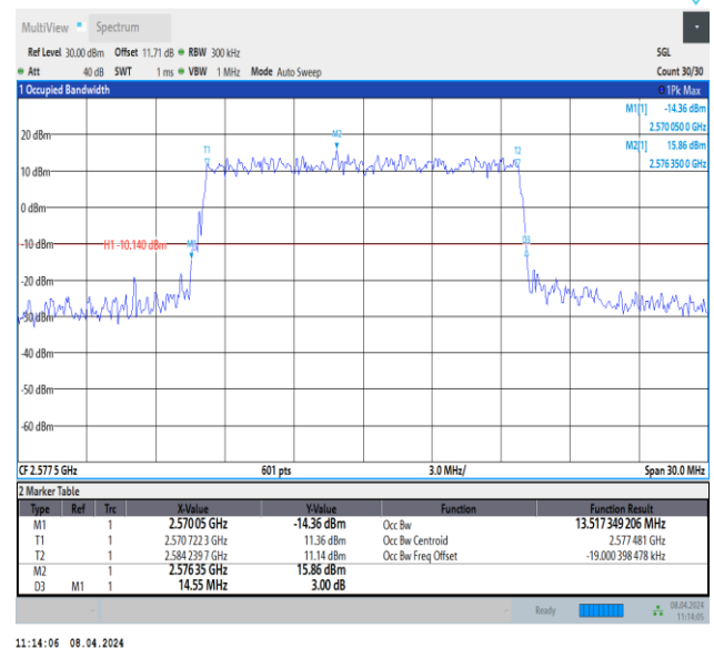
Band38-15MHz-16QAM-37825-75RB#0-PASS
