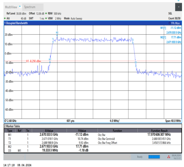
Band41-20MHz-QPSK-41490-100RB#0-PASS
