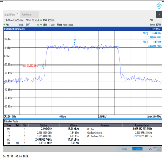
Band41-10MHz-64QAM-39700-50RB#0-PASS
