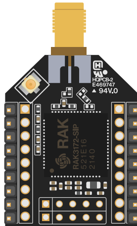
Figure 1: RAK3272-SiP Breakout Board top view
