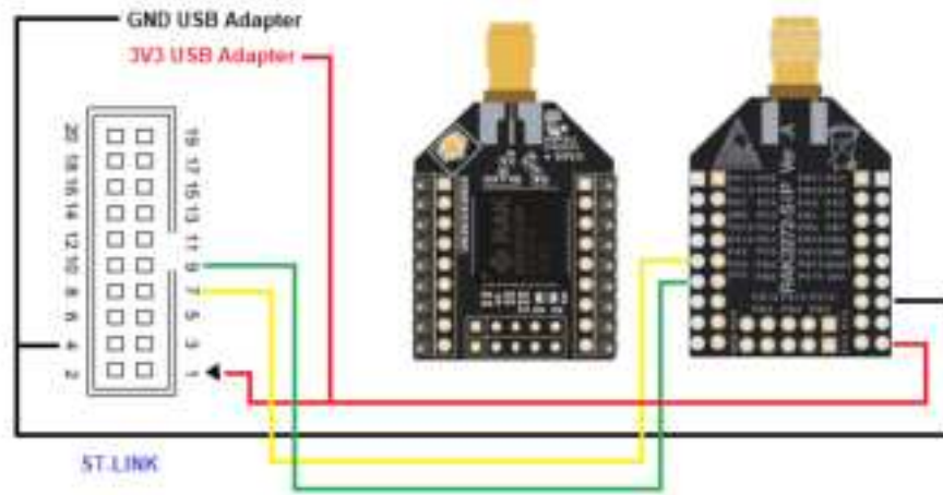
Figure 9: RAK3272-SiP Breakout Board ST-Link connection
