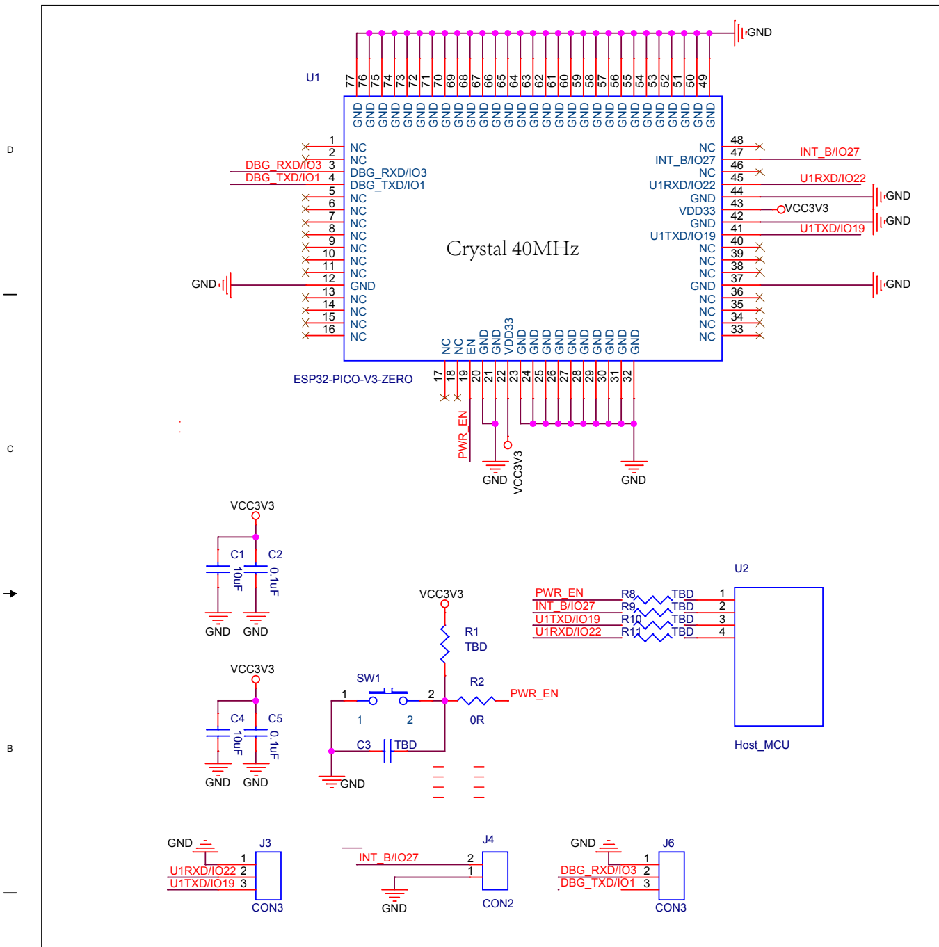
Figure 3: ESP32-PICO-V3-ZERO Module Peripheral Schematics
