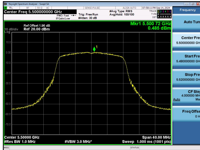
802.11a-Ant1-5500-PASS
