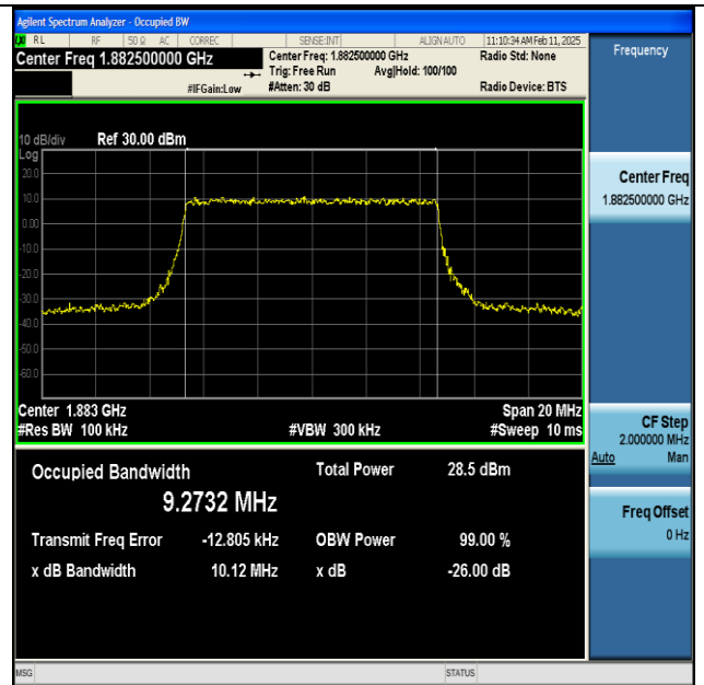
NTNV-n25-PC3-15-10-M-CP-QPSK-Outer_Full-Ant1-PASS
