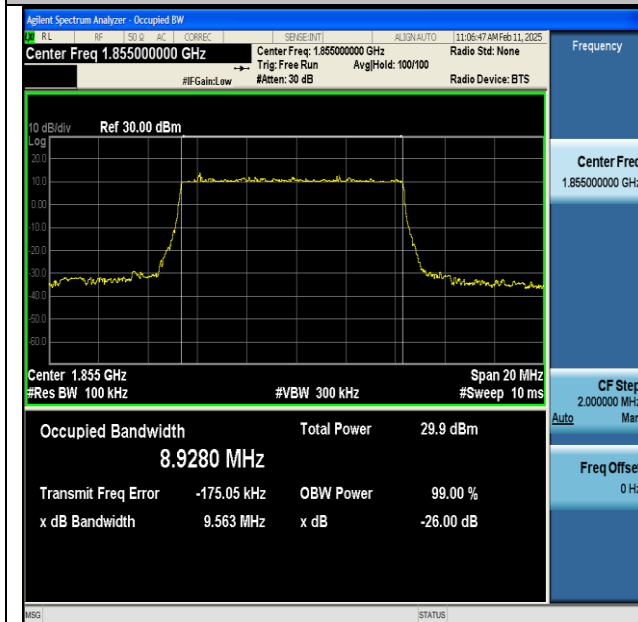
NTNV-n25-PC3-15-10-L-DFT-64QAM-Outer_Full-Ant1- PASS
