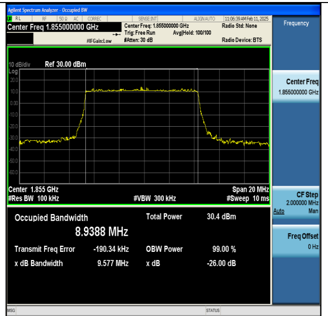
NTNV-n25-PC3-15-10-L-DFT-16QAM-Outer_Full-Ant1- PASS
