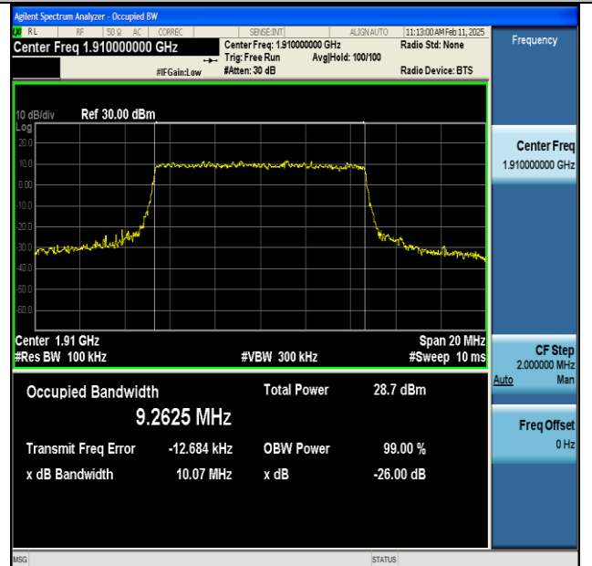
NTNV-n25-PC3-15-10-H-CP-16QAM-Outer_Full-Ant1- PASS
