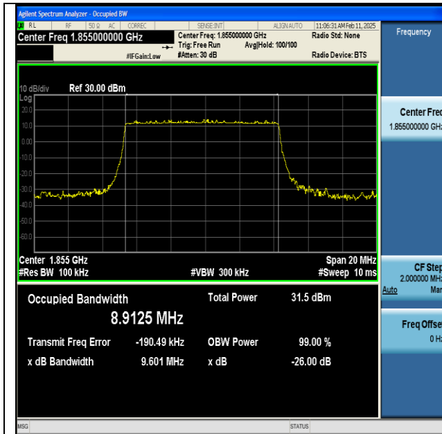
NTNV-n25-PC3-15-10-L-DFT-QPSK-Outer_Full-Ant1- PASS
