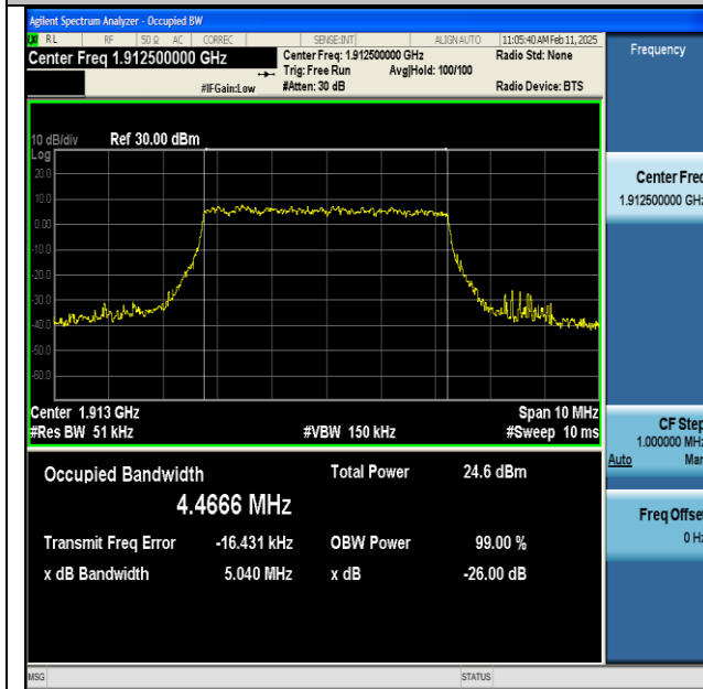
NTNV-n25-PC3-15-5-H-CP-256QAM-Outer_Full-Ant1-PASS
