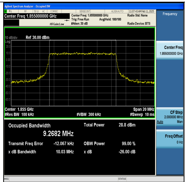
NTNV-n25-PC3-15-10-L-CP-16QAM-Outer_Full-Ant1-PASS
