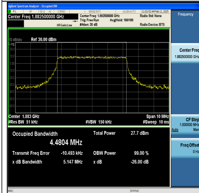
NTNV-n25-PC3-15-5-M-DFT-64QAM-Outer_Full-Ant1- PASS
