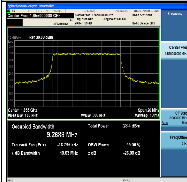
NTNV-n25-PC3-15-10-L-CP-64QAM-Outer_Full-Ant1-PASS
