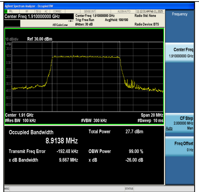
NTNV-n25-PC3-15-10-H-DFT-256QAM-Outer_Full-Ant1- PASS
