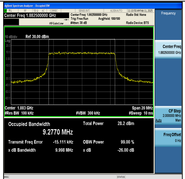
NTNV-n25-PC3-15-10-M-CP-64QAM-Outer_Full-Ant1-PASS
