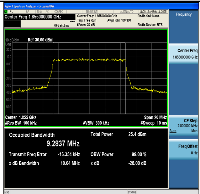
NTNV-n25-PC3-15-10-L-CP-256QAM-Outer_Full-Ant1-PASS
