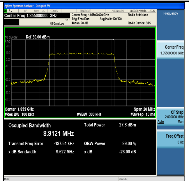
NTNV-n25-PC3-15-10-L-DFT-256QAM-Outer_Full-Ant1- PASS
