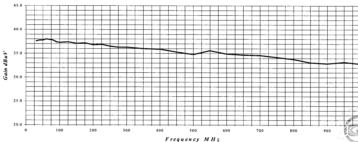
PREAMPLIFIER EFFECTIVE GAIN AT 3 METERS PA-102 S/N: 1017 Effective 1-13-00
