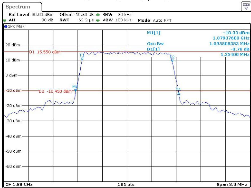
Band 2_1.4 MHz_Middle_QPSK_RB6#0
