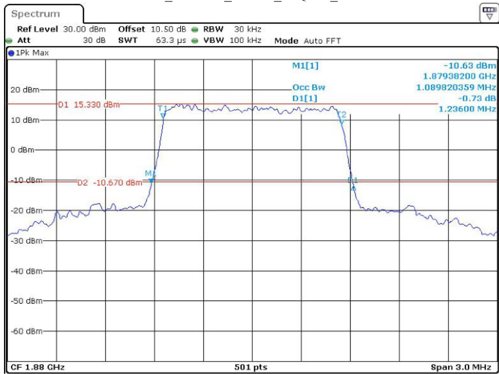
Band 2_1.4 MHz_Middle_16QAM_RB6#0
