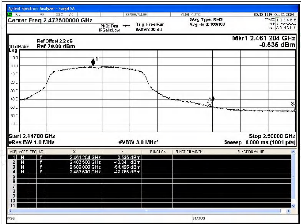
Restrict Band NVNT n20 2462MHz Ant0 Average
