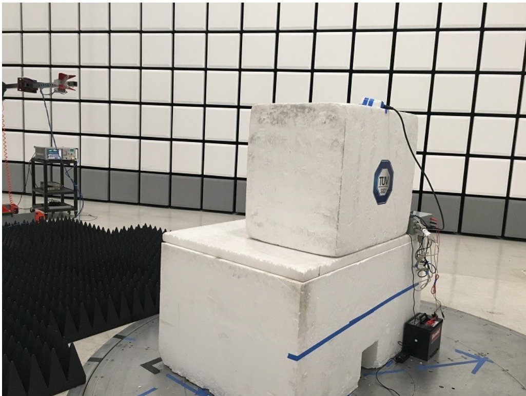
Radiated Emissions Above 1GHz 1GHz Rear
