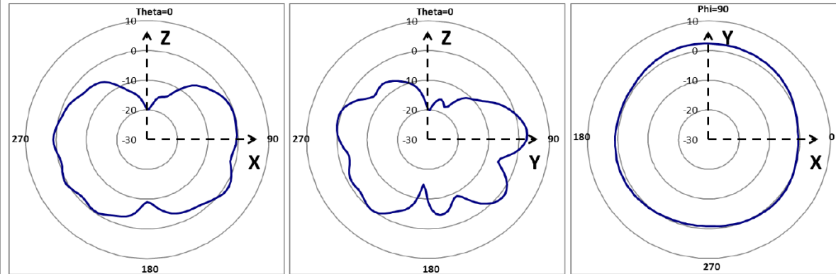
6GHz Radiation Pattern
