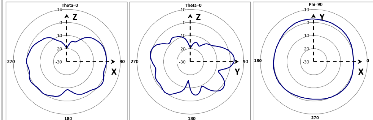
6GHz Radiation Pattern
