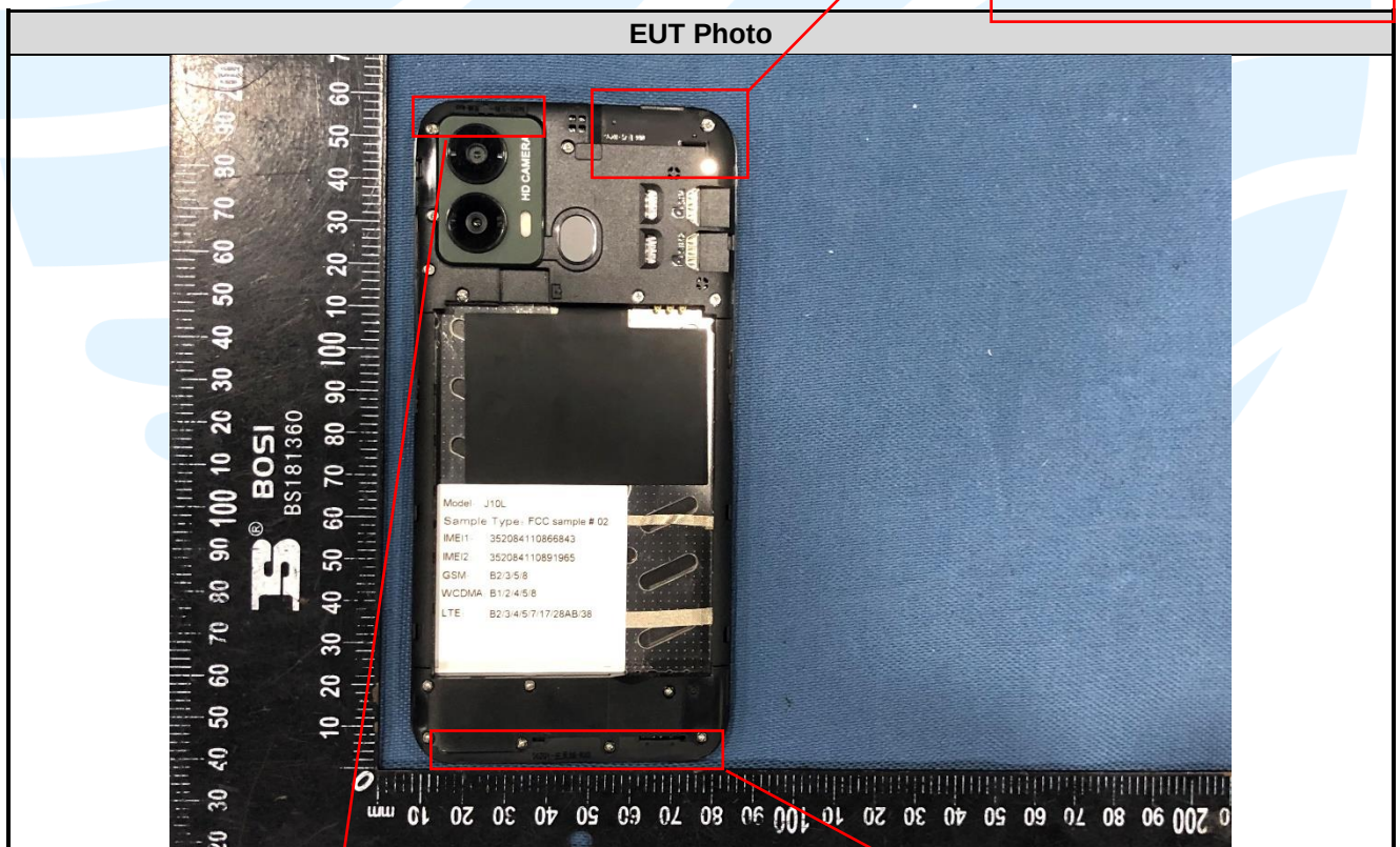
WLAN/BT/GPS Antenna
