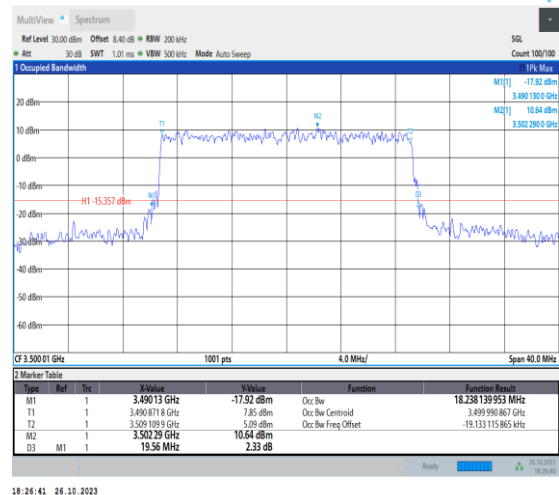
1-N78-3450-3550-PC2-30-20-M-6-CP-QPSK-Outer_Full-51@0-Ant0-18.238-19.560-≤20-PASS
