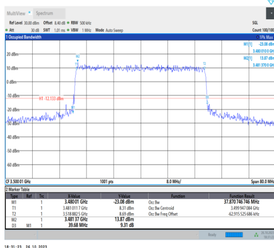
1-N78-3450-3550-PC2-30-40-M-8-CP-64QAM-Outer_Full-106@0-Ant0-37.871-39.680-≤40-PASS
