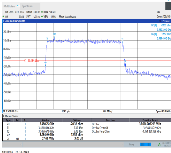
1-N78-3450-3550-PC2-30-40-M-5-DFT-256QAM-Out er_Full-100@0-Ant0-35.618-37.680-≤40-PASS
