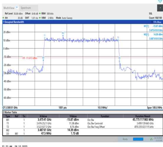
1-N78-3450-3550-PC2-30-50-M-2-DFT-PI2BPSK-Outer _Full-128@0-Ant0-45.775-47.500-≤50-PASS
