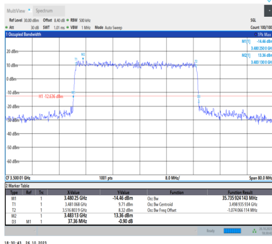
1-N78-3450-3550-PC2-30-40-M-4-DFT-64QAM-Outer_Full-100@0-Ant0-35.736-37.360-≤40-PASS
