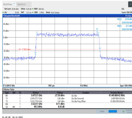
1-N78-3450-3550-PC2-30-50-M-9-CP-256QAM-Outer_Full-133@0-Ant0-47.446-49.500-≤50-PASS
