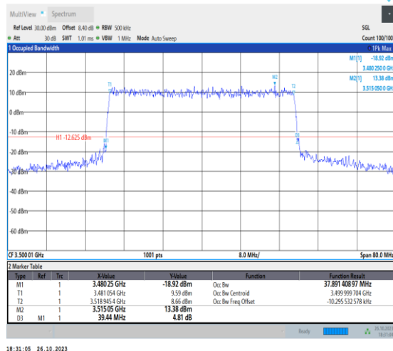
1-N78-3450-3550-PC2-30-40-M-6-CP-QPSK-Outer_Full-106@0-Ant0-37.891-39.440-≤40-PASS
