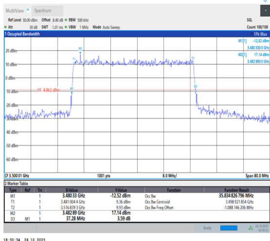
1-N78-3450-3550-PC2-30-40-M-3-DFT-16QAM-Outer_Full-100@0-Ant0-35.835-37.280-≤40-PASS
