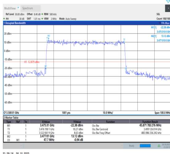
1-N78-3450-3550-PC2-30-50-M-3-DFT-16QAM-Outer _Full-128@0-Ant0-45.872-47.700-≤50-PASS
