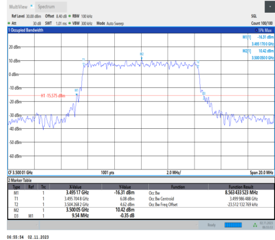
1-N78-3450-3550-PC2-30-10-M-2-DFT-PI2BPSK-Out _Full-24@0-Ant1-8.563-9.540-≤10-PASS
