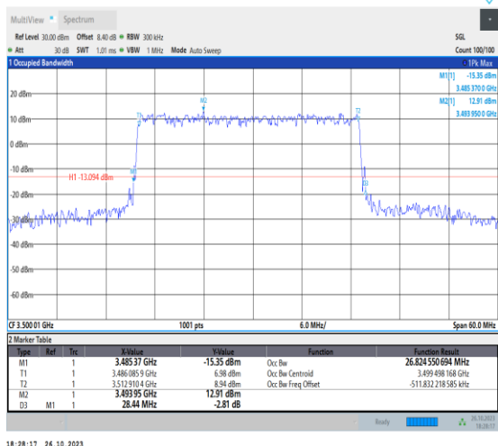
1-N78-3450-3550-PC2-30-30-M-4-DFT-64QAM-Outer_Full-75@0-Ant0-26.825-28.440-≤30-PASS
