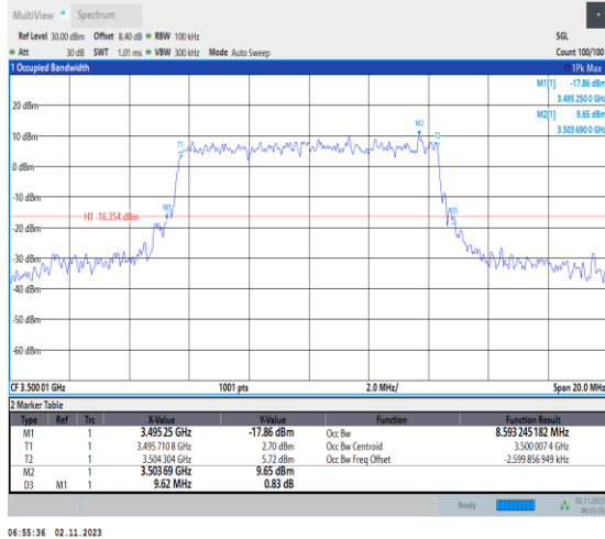
1-N78-3450-3550-PC2-30-10-M-1-DFT-QPSK-Out _Full-24@0-Ant1-8.593-9.620-≤10-PASS
