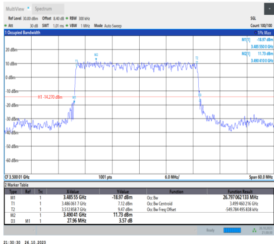
1-N78-3450-3550-PC2-30-30-M-2-DFT-PI2BPSK-Outer_Full-75@0-Ant0-26.797-27.960-≤30-PASS
