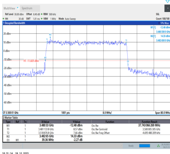
1-N78-3450-3550-PC2-30-40-M-7-CP-16QAM-Outer_Full-106@0-Ant0-37.743-39.360-≤40-PASS
