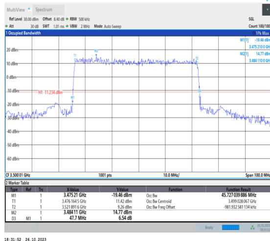
1-N78-3450-3550-PC2-30-50-M-1-DFT-QPSK-Outer _Full-128@0-Ant0-45.727-47.700-≤50-PASS
