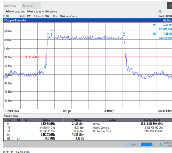
1-N78-3450-3550-PC2-30-40-M-2-DFT-PI2BPSK-Outer_Full-100@0-Ant0-35.813-38.000-≤40-PASS
