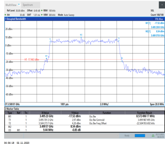
1-N78-3450-3550-PC2-30-10-M-4-DFT-64QAM-Out _Full-24@0-Ant1-8.572-9.440-≤10-PASS
