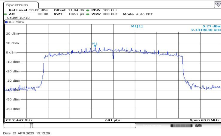
11AX40-CDD_Ant4_2447_0~Reference
