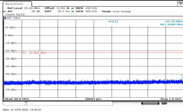
11BE20-CDD_Ant3_2457_30~1000
