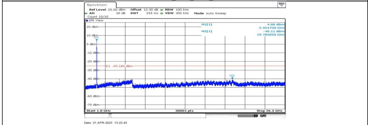
11AX40-CDD_Ant2_2452_1000~26500
