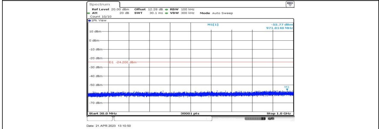
11AX40-CDD_Ant2_2447_30~1000
