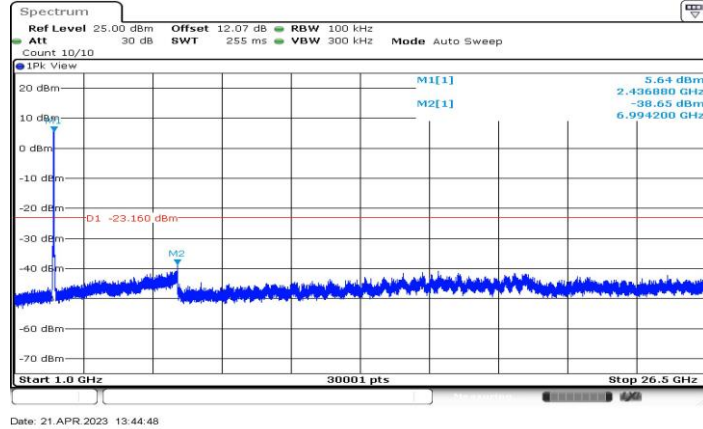
11AX40-CDD_Ant1_2437_1000~26500
