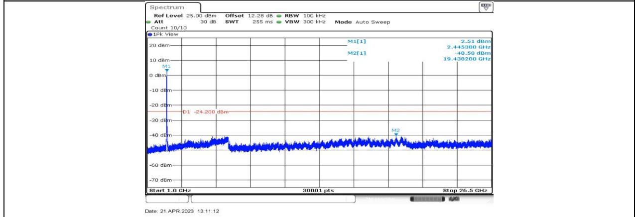
11AX40-CDD_Ant2_2447_1000~26500
