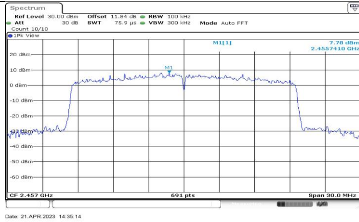
11BE20-CDD_Ant3_2457_0~Reference
