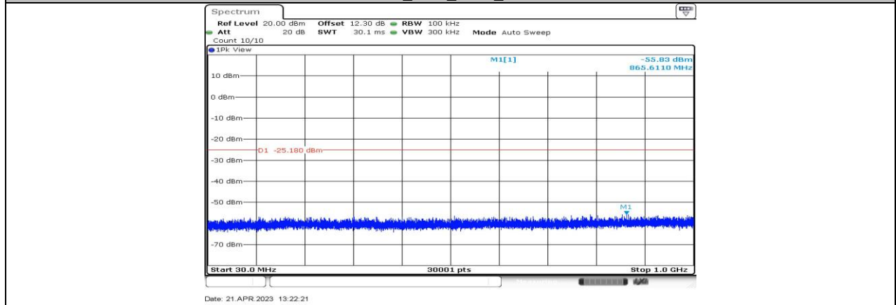
11AX40-CDD_Ant2_2452_30~1000
