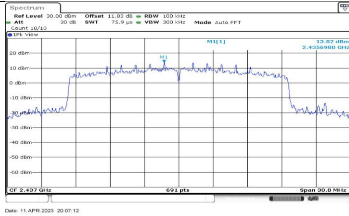
11BE20-CDD_Ant3_2437_0~Reference
