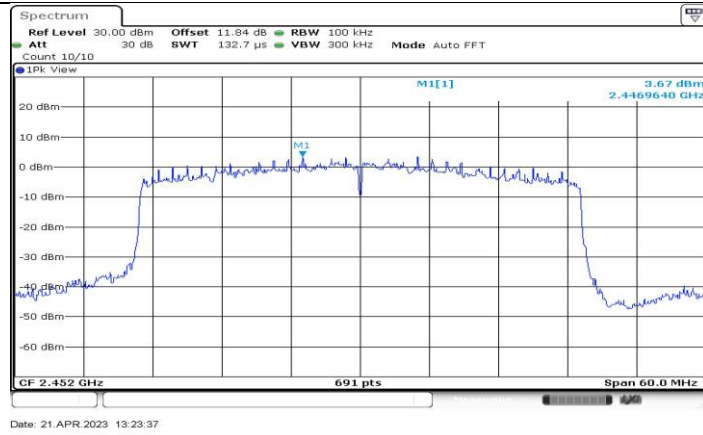
11AX40-CDD_Ant3_2452_0~Reference
