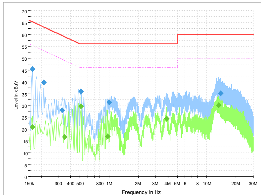
Fig.A.6.2. AC Powerline Conducted Emission-Iidle
