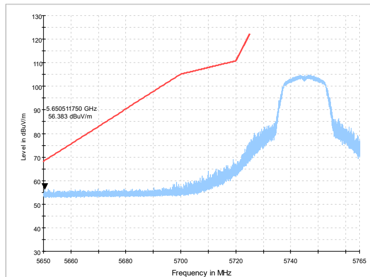
Fig. 1 Band Edges (802.11a Ch149,5745MHz)
