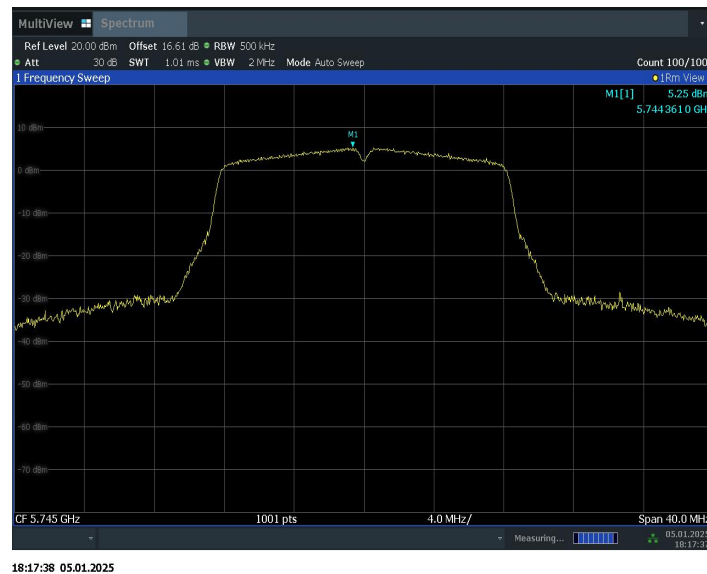
Peak Power Spectral Density:11a CH149
