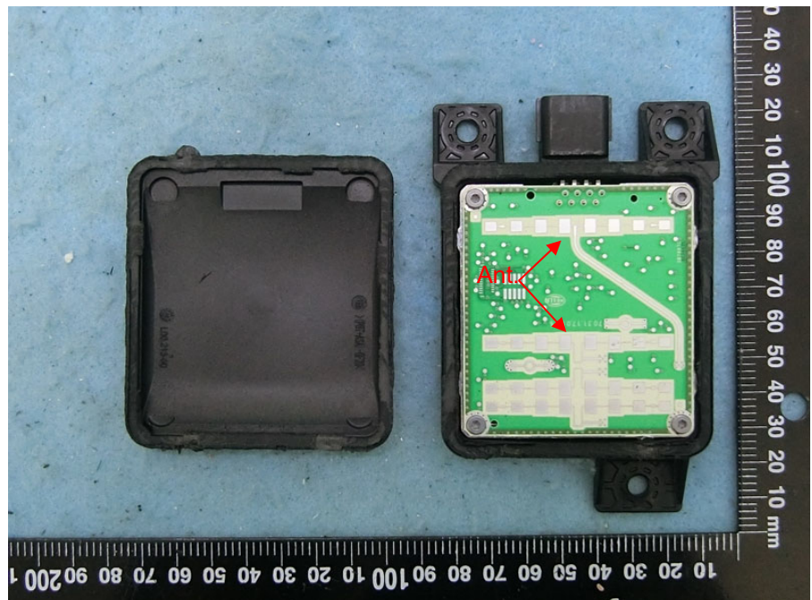
Slave Control Unit (EUT)
