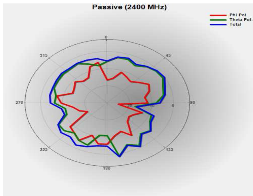
2400 MHz Azimuth 90°
