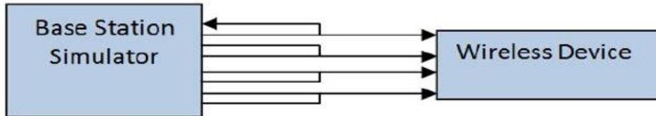
Figure: Power Measurement setup for Carrier Aggregation Scenarios with 2 Component Carriers with 4x4 DL-MIMO
