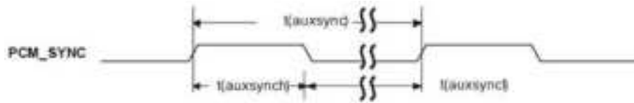
Figure 25: PCM_SYNC timing
