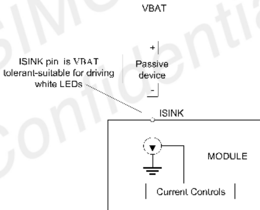
Figure 34: ISINK reference circuit
