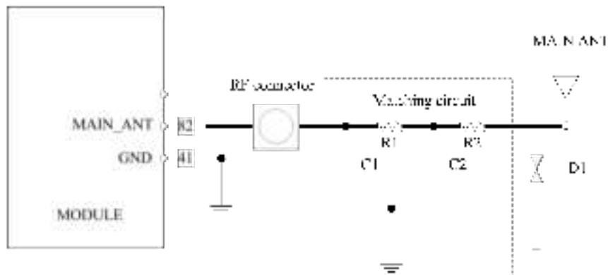
Figure 35: Antenna matching circuit (MAIN_ANT)
