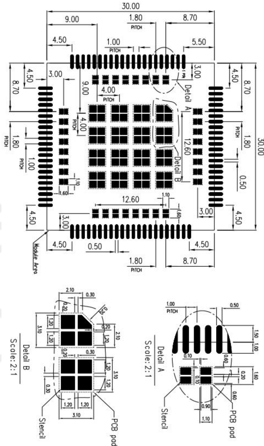
Figure 42 : Stencil Foil
