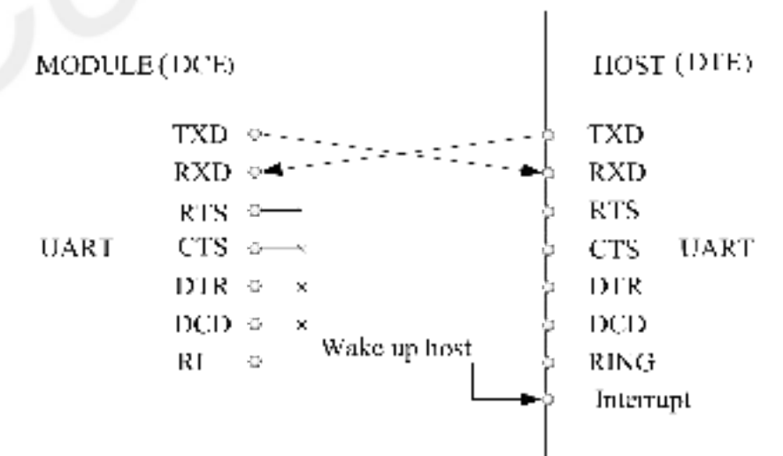
Figure 14: UART null modem
