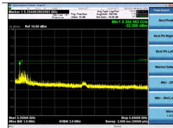
802.11ax20 | Channel 64 | MCS0 | RU52 | Peak
