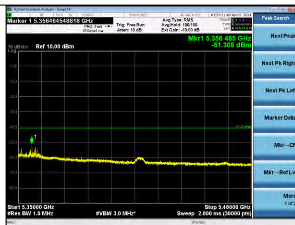
802.11ax20 | Channel 64 | MCS0 | RU52 | Average
