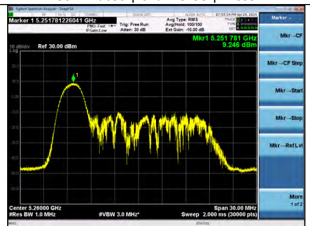
802.11ax20 | Channel 52 | MCS0 | RU26
