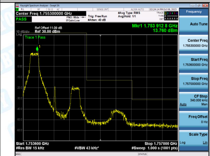
Band4_1.4MHz_16QAM_20393_1RB#0
