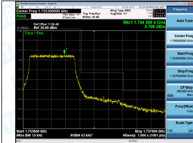
Band4_1.4MHz_QPSK_20393_6RB#0
