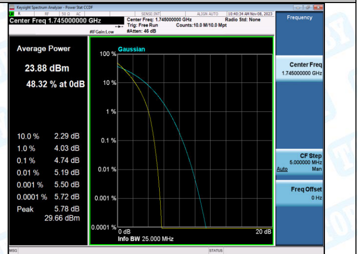
Band4-20MHz-QPSK-20300-100RB#0-PASS
