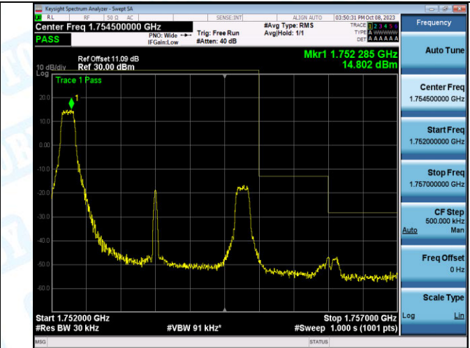
Band4_3MHz_16QAM_20385_1RB#0
