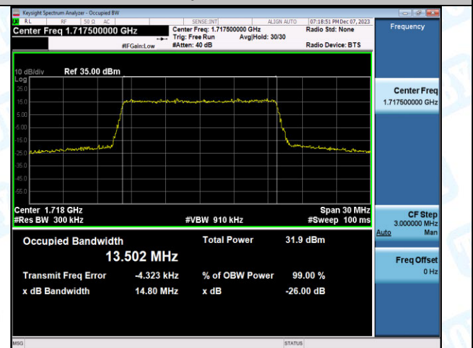
Band4-15MHz-QPSK-20325-75RB#0-PASS
