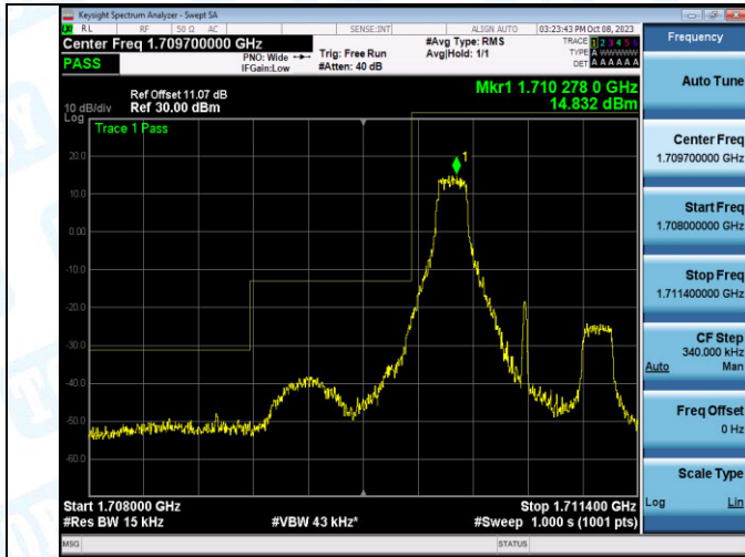
Band4_1.4MHz_QPSK_19957_1RB#0
