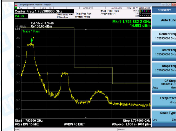
Band4_1.4MHz_QPSK_20393_1RB#0
