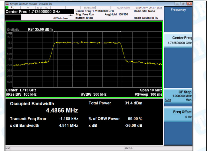
Band4-5MHz-16QAM-20175-25RB#0-PASS
