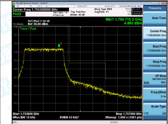
Band4_1.4MHz_16QAM_20393_6RB#0
