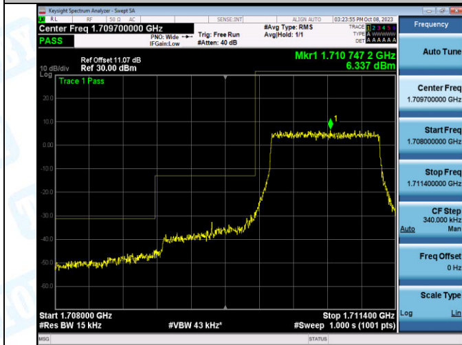
Band4_1.4MHz_QPSK_19957_6RB#0
