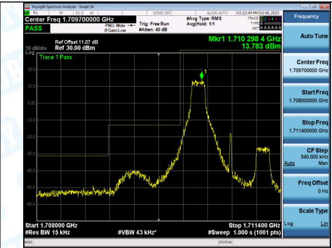
Band4_1.4MHz_16QAM_19957_1RB#0
