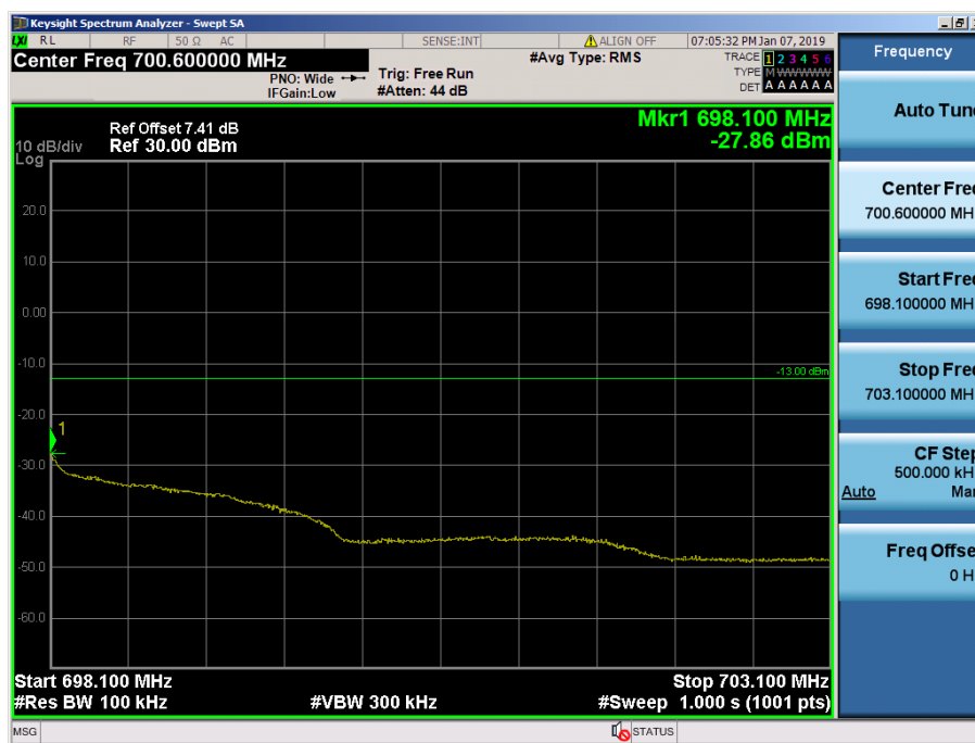
LTE Band 71 / 5MHz / QPSK - RB Size/Offset (12/13)
