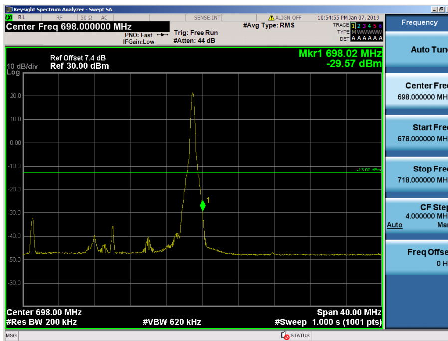
LTE Band 71 / 20MHz / 16QAM - RB Size/Offset (1/99)
