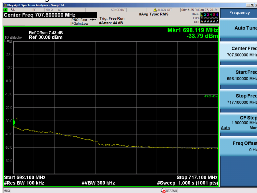
LTE Band 71 / 20MHz / QPSK - RB Size/Offset (50/50)
