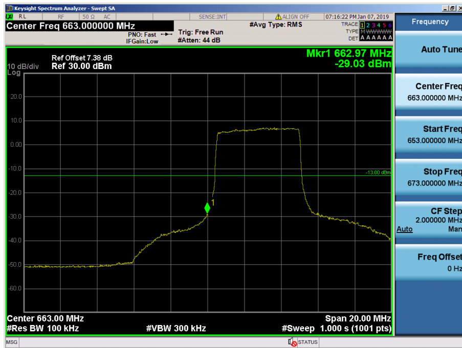
LTE Band 71 / 10MHz / QPSK - RB Size/Offset (25/0)
