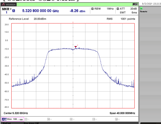
[ 802.11a/ 5320 MHz ]
