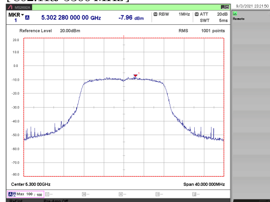
[ 802.11a/ 5300 MHz ]
