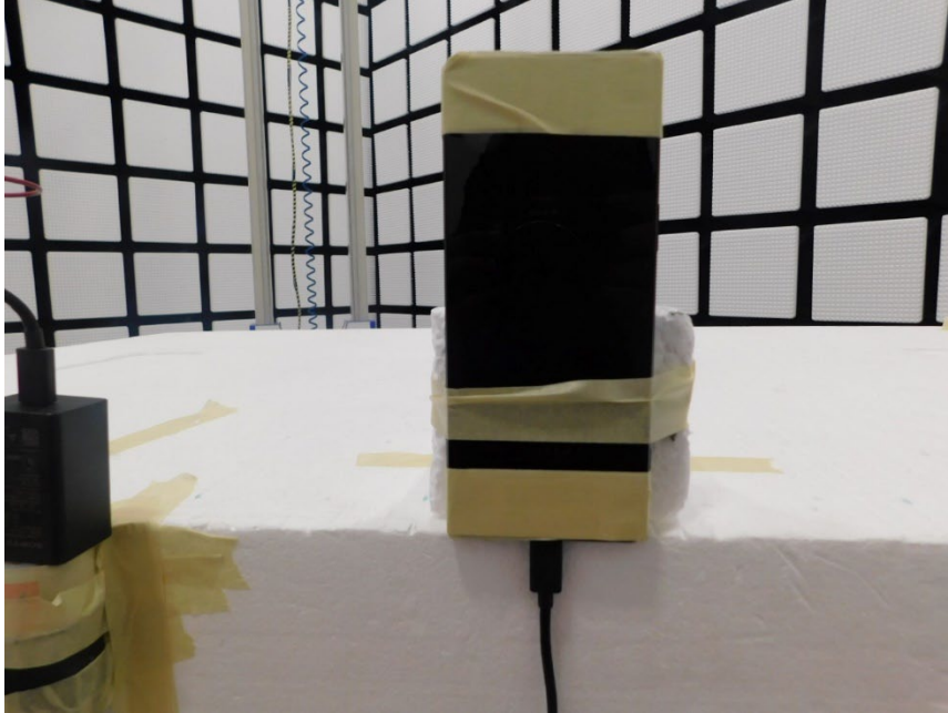
Z-ORIENTATION (Configuration 1)
