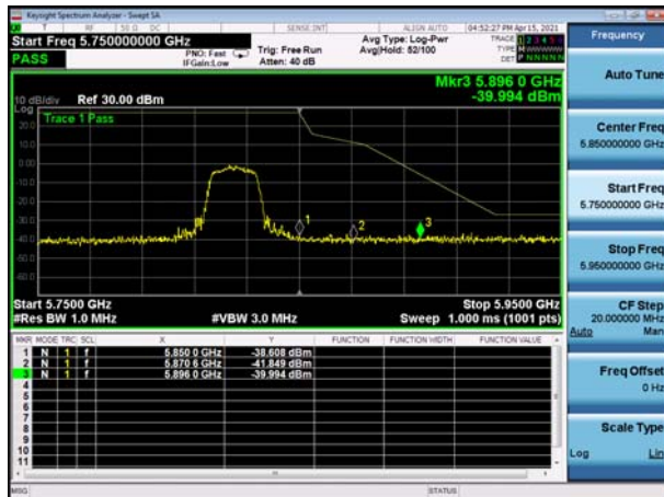
U-NII-3 ,Plot 1,Band Edge-802.11ac(20 MHz),5785MHz,Ant1
