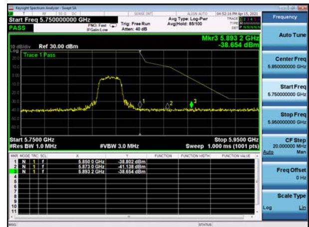
U-NII-3 ,Plot 1,Band Edge-802.11ac(20 MHz),5825MHz,Ant1
