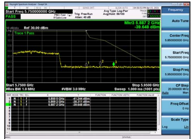
U-NII-3 ,Plot 1,Band Edge-802.11ac(80 MHz),5775MHz,Ant1 BandEdge Right
