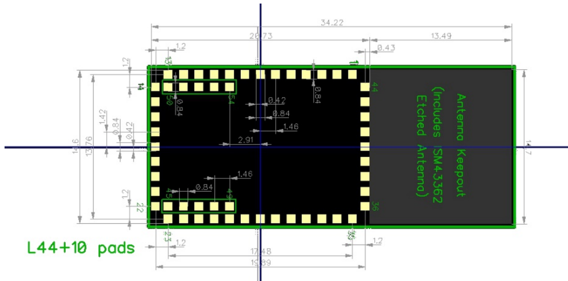
"Keep out" area should have the antenna hanging off the side of the PCB for best performance. If you do not hang the antenna off the PCB, remove ground planes and PCB material under the antenna (13.49 x 14.7 mm keep out area). Surrounding metal should be 9 mm away from cutout area, metal will affect the antenna performance. The external antenna does not require "keep out" area.
