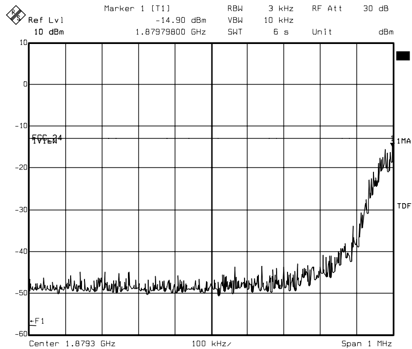
diagram 8.09: carrier on channel 661 (1880 MHz), TCH mode
