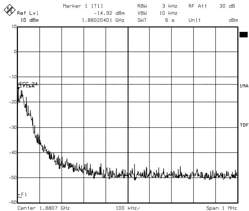
diagram 8.10: carrier on channel 661 (1880 MHz), TCH mode
