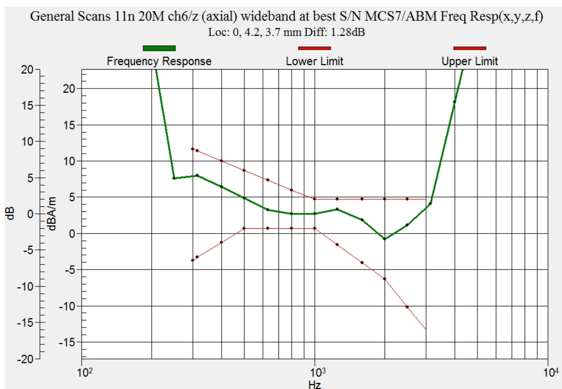
Figure C.19 Frequency Response of WiFi-2.4G
