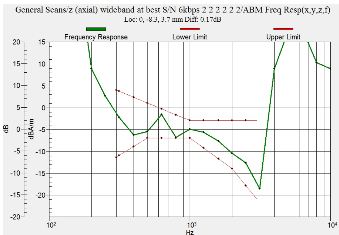
Figure C.20 Frequency Response of GSM1900 - OTT VoIP
