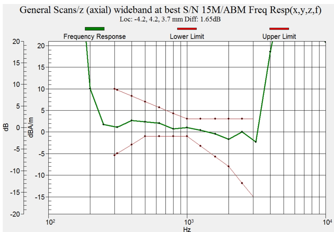
Figure C.14 Frequency Response of LTE B25
