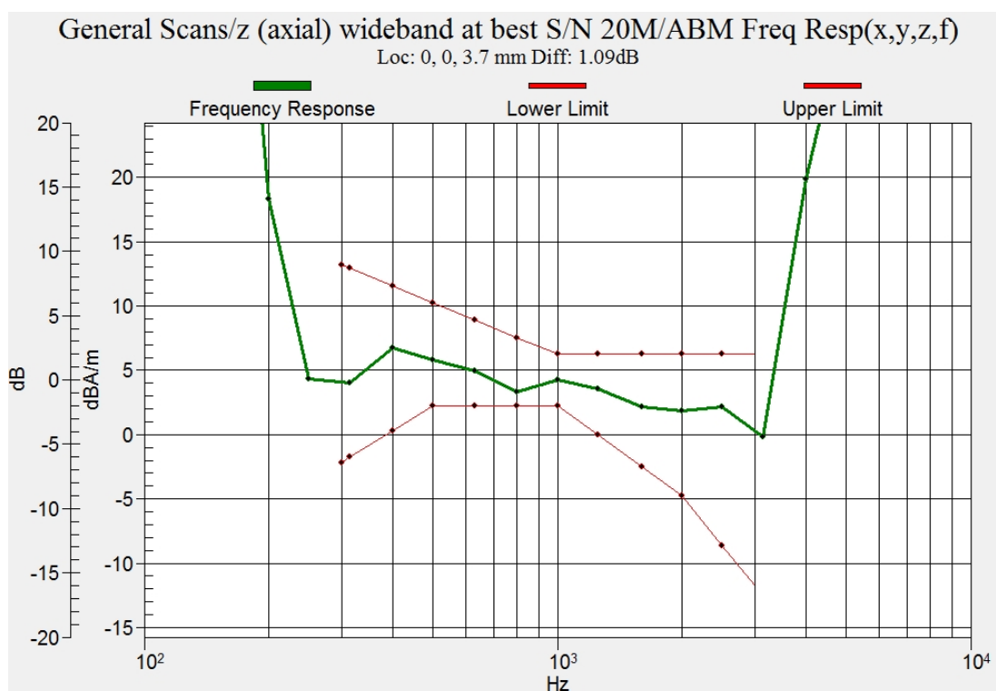
Figure C.16 Frequency Response of LTE B41 Power Class 2
