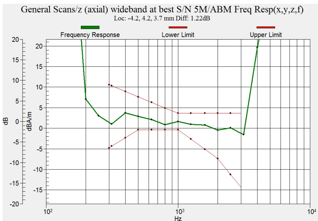
Figure C.12 Frequency Response of LTE B12
