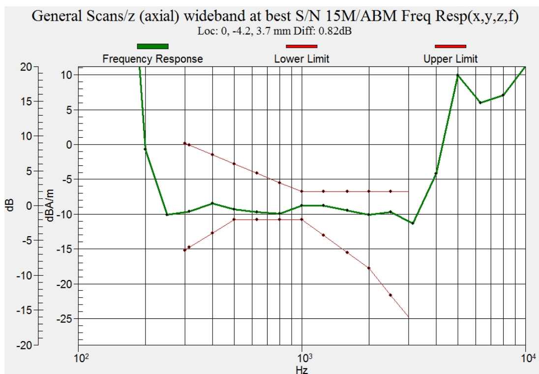
Figure C.15 Frequency Response of LTE B26
