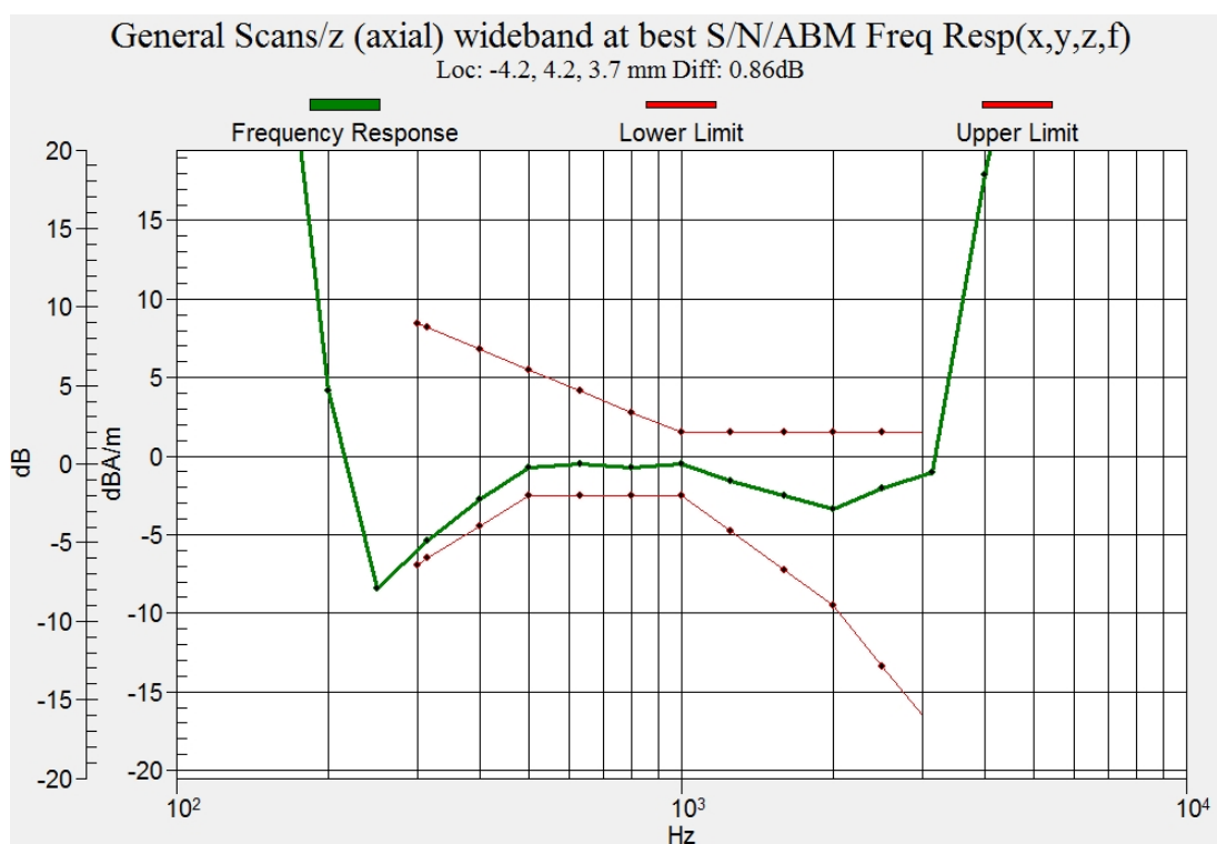
Figure C.5 Frequency Response of WCDMA 1700
