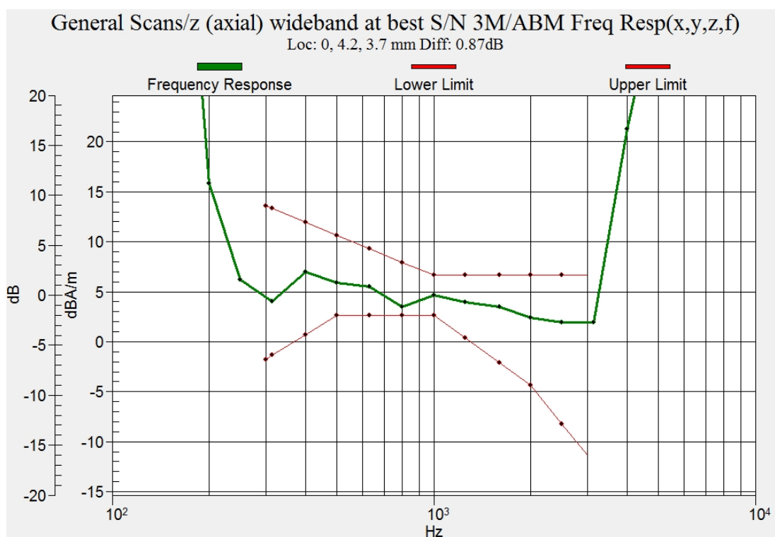
Figure C.11 Frequency Response of LTE B5
