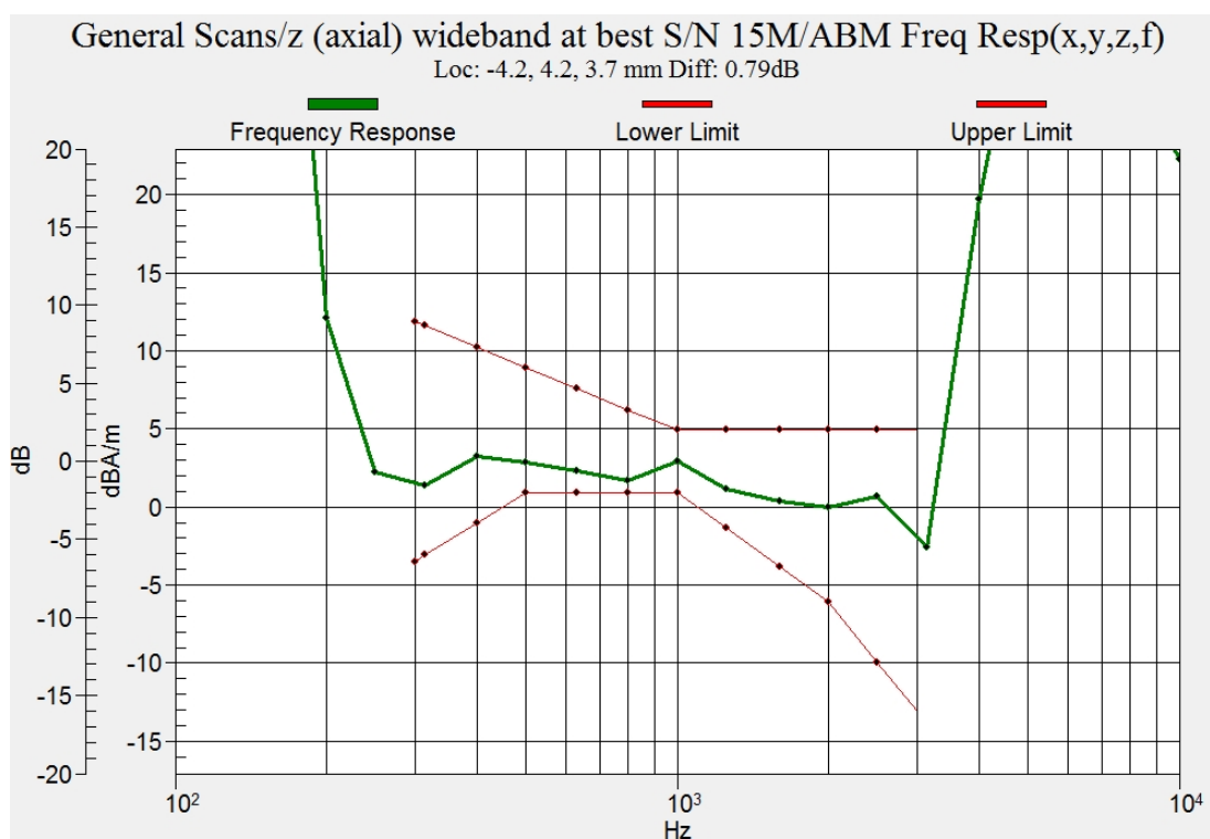
Figure C.9 Frequency Response of LTE B2
