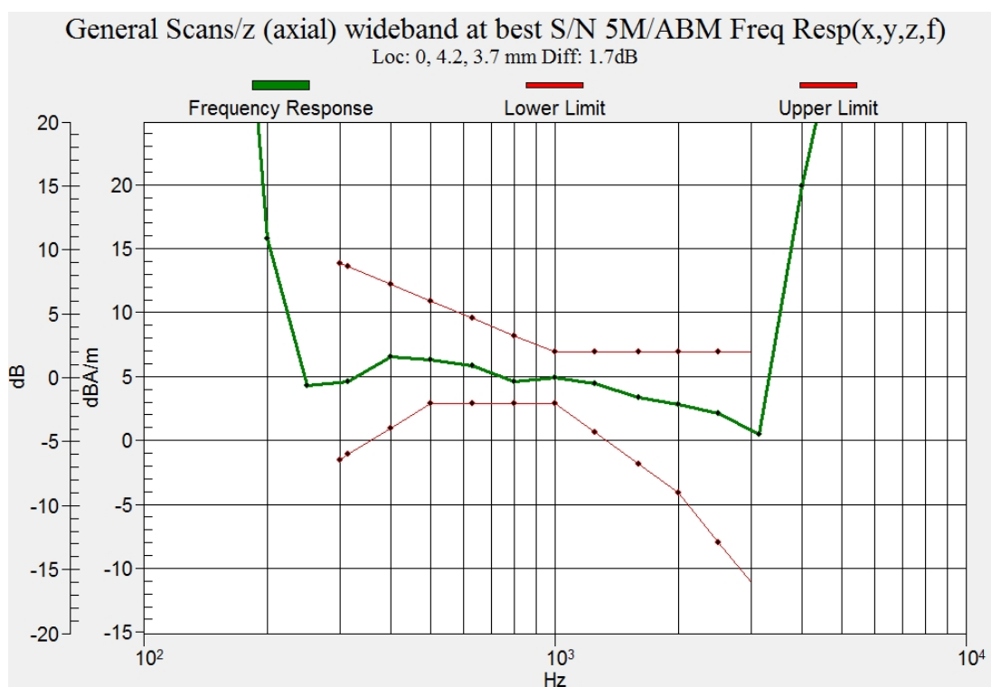
Figure C.13 Frequency Response of LTE B13
