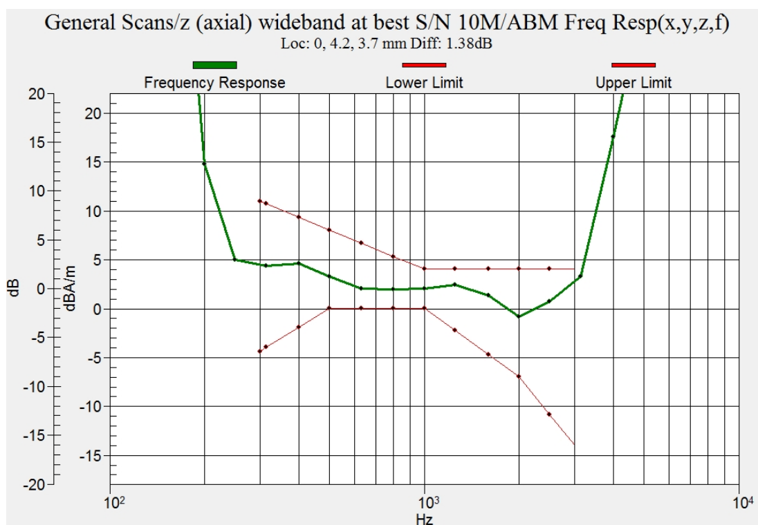
Figure C.18 Frequency Response of LTE B71
