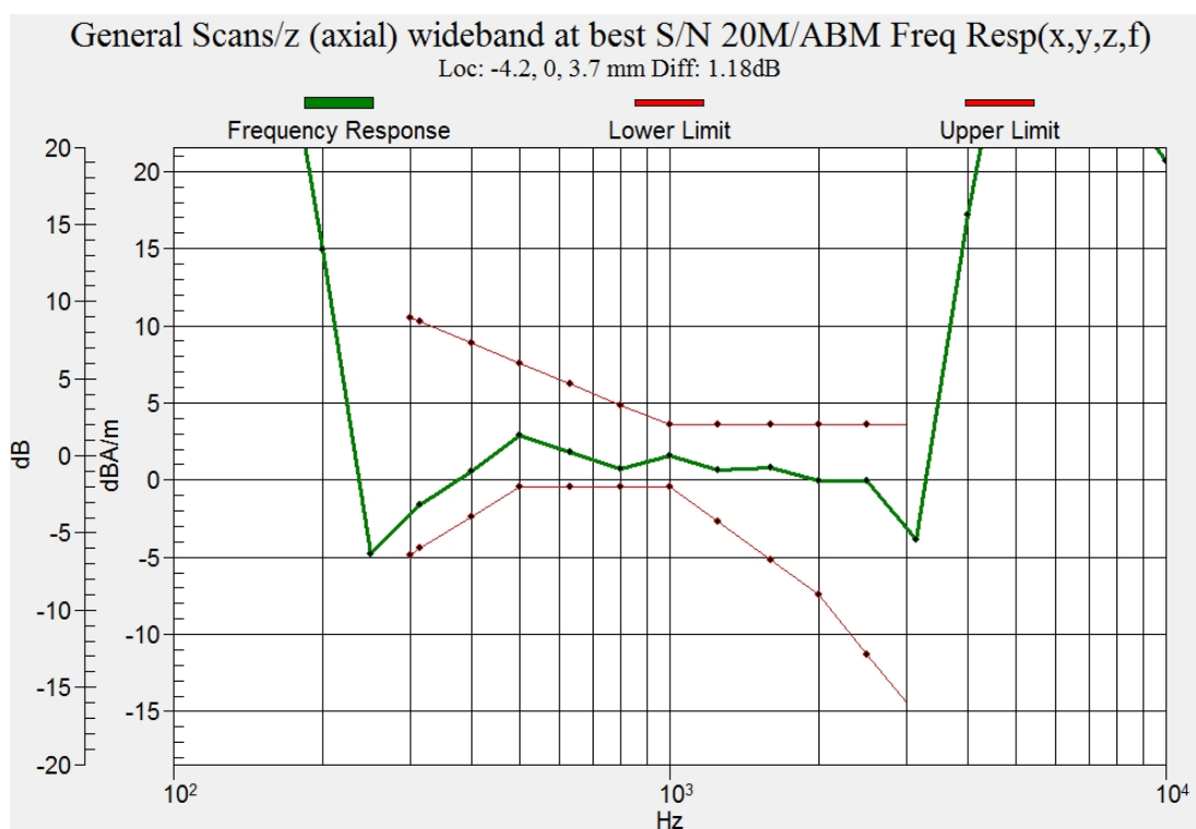
Figure C.17 Frequency Response of LTE B41 Power Class 3
