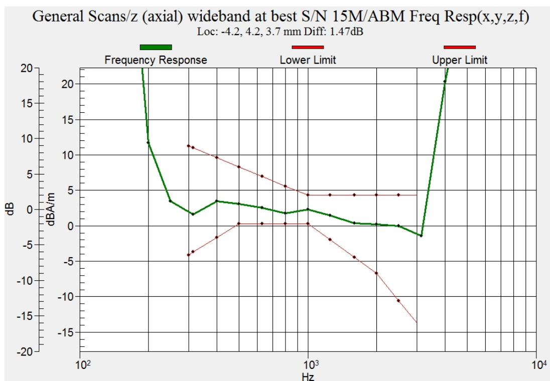
Figure C.10 Frequency Response of LTE B4
