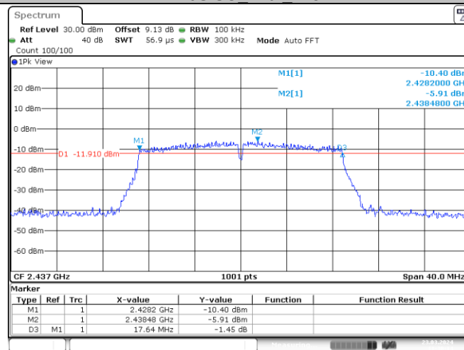
11N20SISO Ant1_2437
