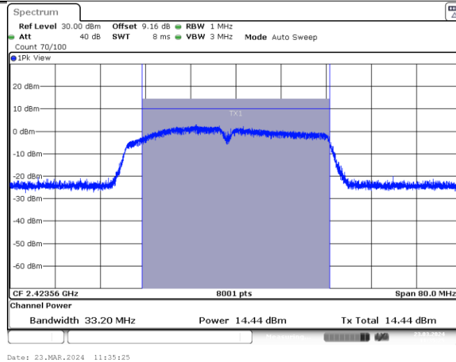
11N40SISO Ant1_2437
