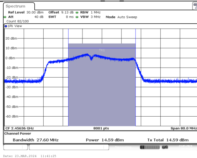
11N40SISO Ant1_2452
