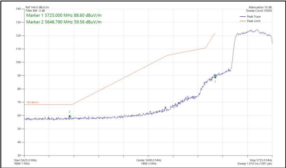
Figure 463 - 802.11ax HE20, SU, SDM, Core 0 - Core 1 - 5745 MHz Band Edge Frequency 5725 MHz
