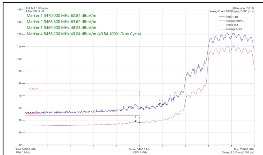
Figure 428 - 802.11ax HE20, SU, CDD, Core 0 - Core 1 - 5500 MHz Band Edge Frequency 5470 MHz
