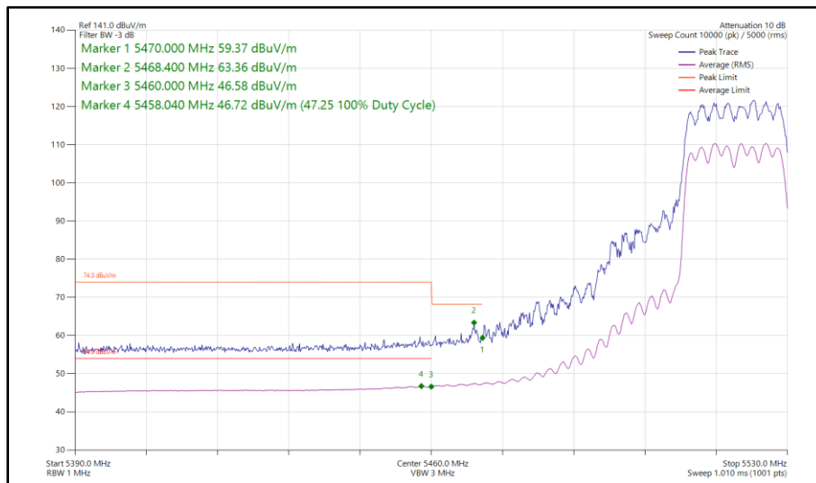
Figure 430 - 802.11ax HE20, SU, CDD, Core 0 - Core 1 - 5520 MHz Band Edge Frequency 5470 MHz
