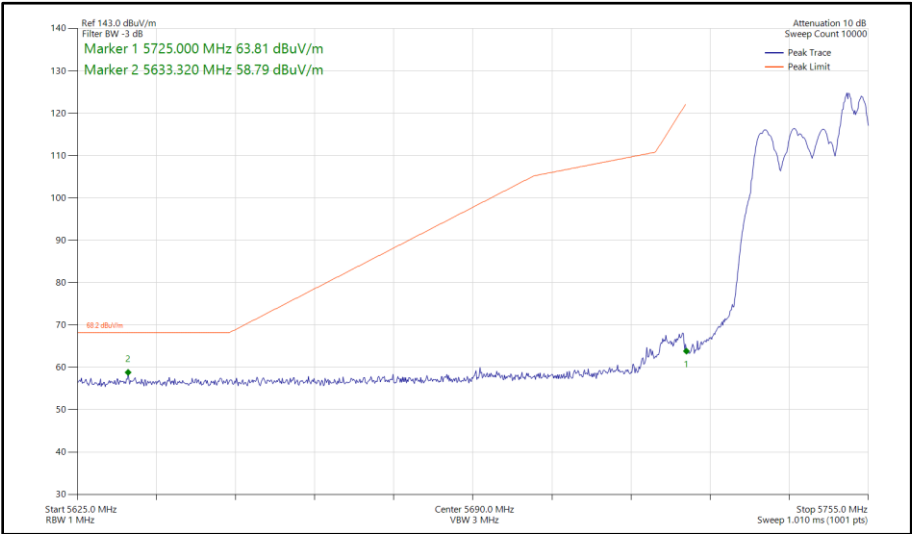
Figure 436 - 802.11ax HE20, RU 52-40, CDD, Core 0 - Core 1 - 5745 MHz Band Edge Frequency 5725 MHz
