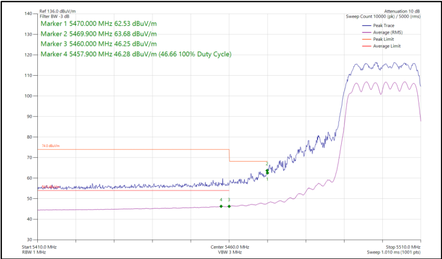
Figure 426 - 802.11n HT20, CDD, Core 0 - Core 1 - 5500 MHz Band Edge Frequency 5470 MHz
