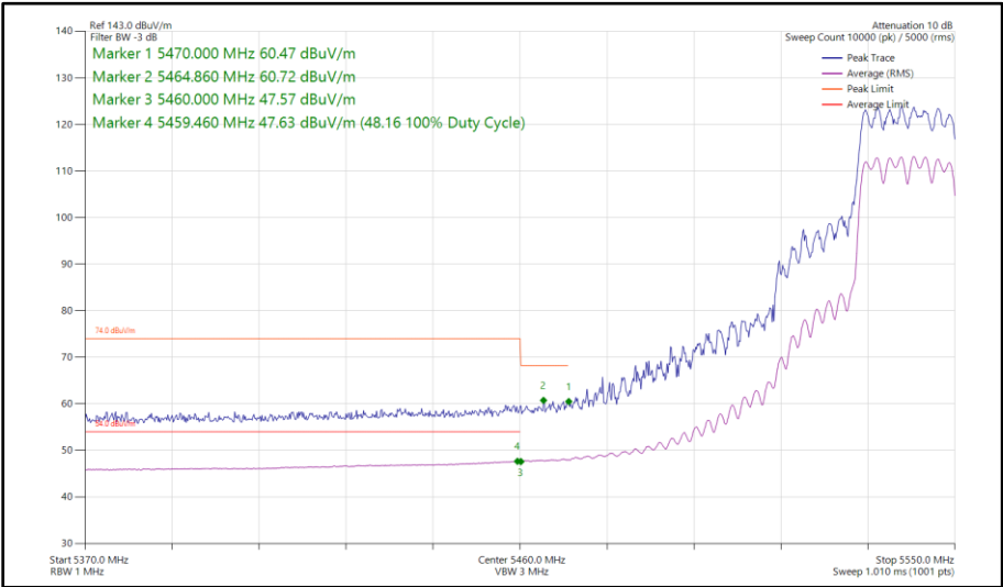
Figure 432 - 802.11ax HE20, SU, CDD, Core 0 - Core 1 - 5540 MHz Band Edge Frequency 5470 MHz
