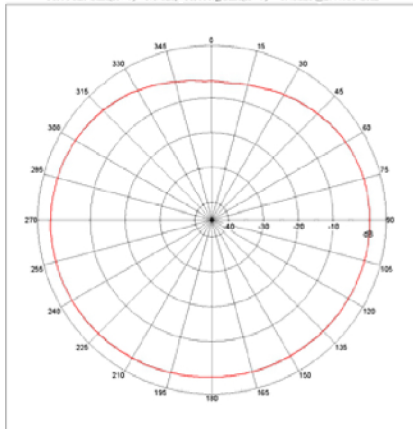
Far-field Power Distribution(H+V) on X-Y Plane Plot Peak Gain(H+V)= 1.7 dB; Plot AvgGain(H+V)= -0.45dB @2.44000 GHz
