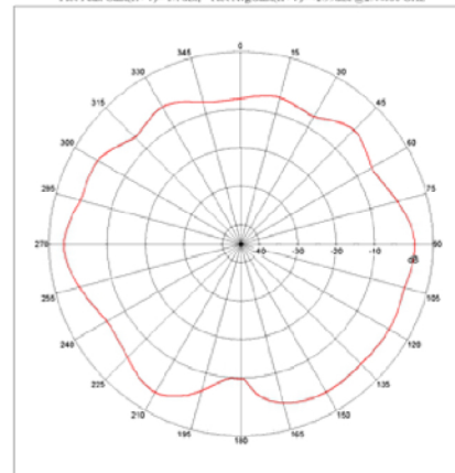
Far-field Power Distribution(H+V) on Y-Z Plane Plot Peak Gain(H+V)= 1.1 dB; Plot AvgGain(H+V)= -2.99dB @2.44000 GHz
