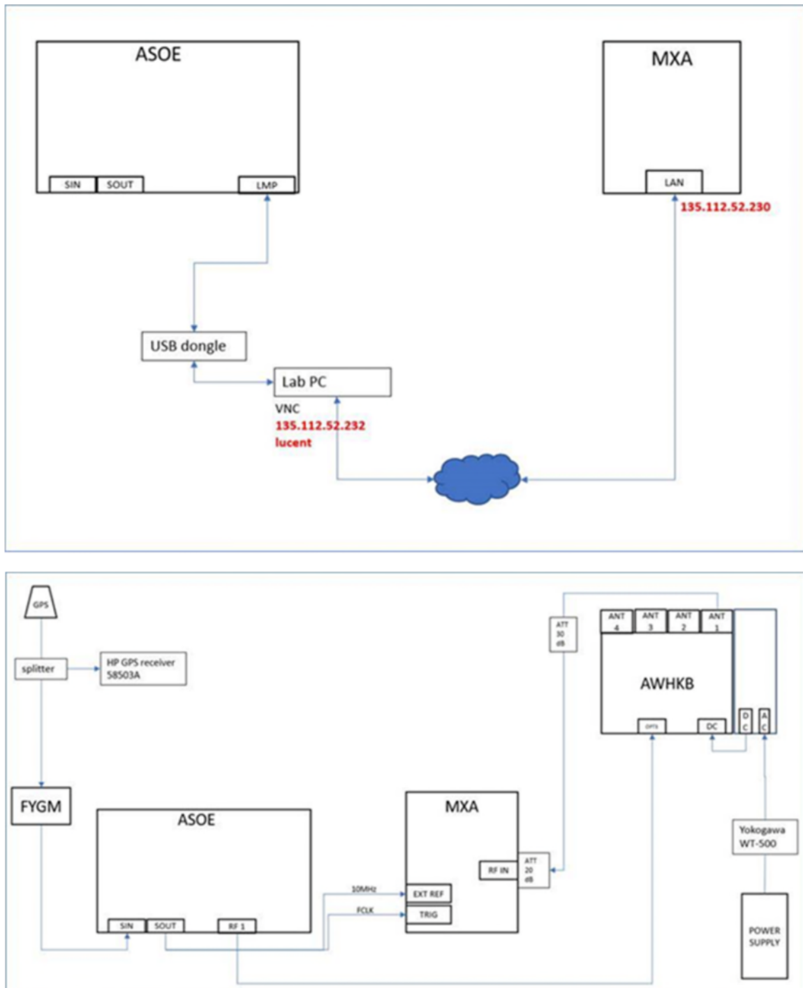
Figure 3. Frequency Stability Test
