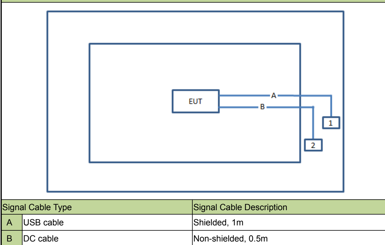
Connection Diagram
