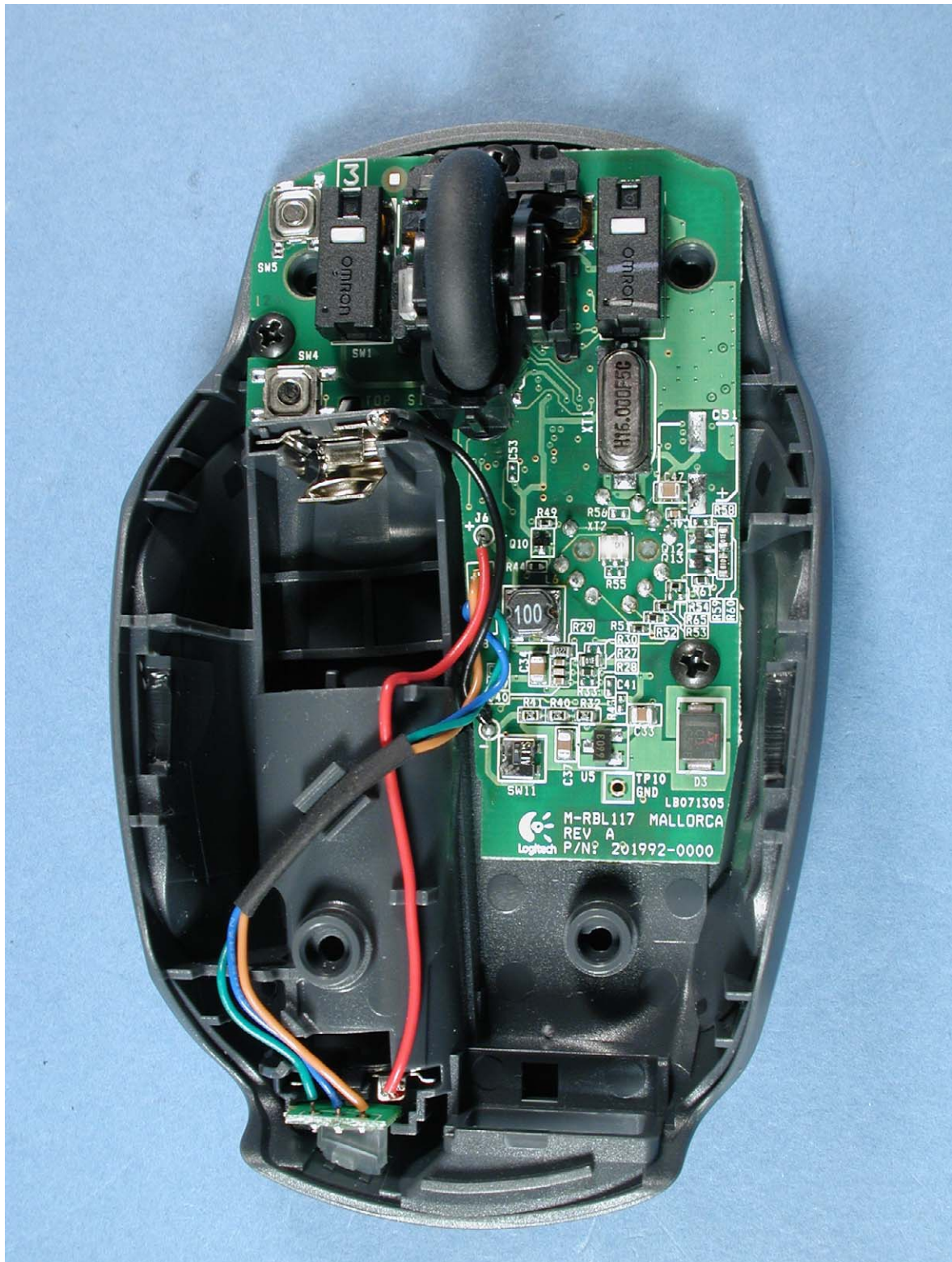
Photograph 6: M-RBL117 interior view
