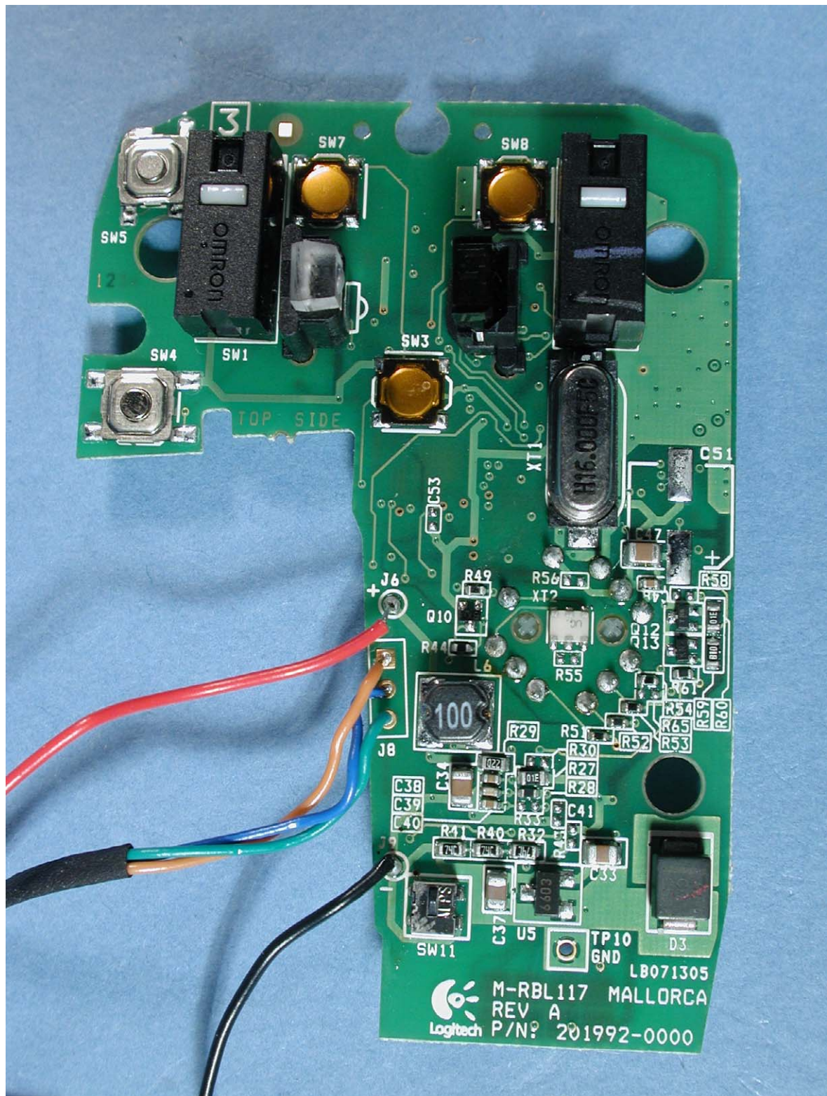
Photograph 7: M-RBL117 top view PCB
