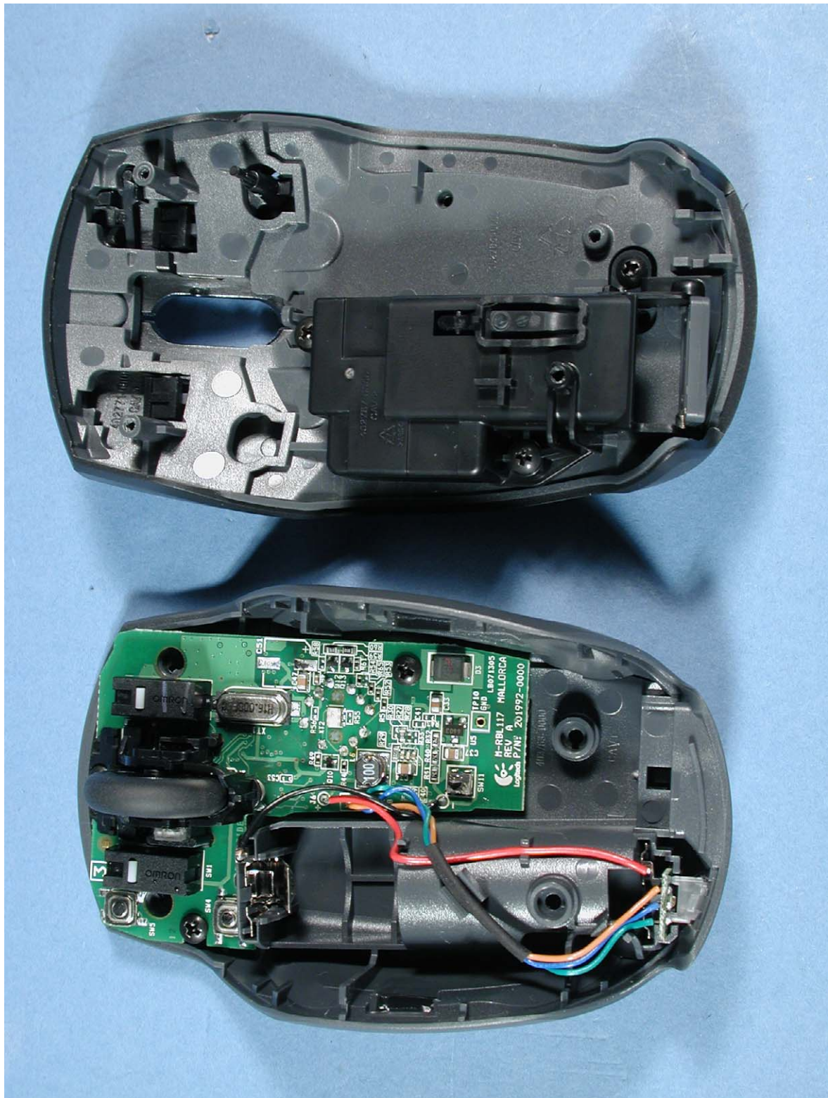
Photograph 5: M-RBL117 interior view
