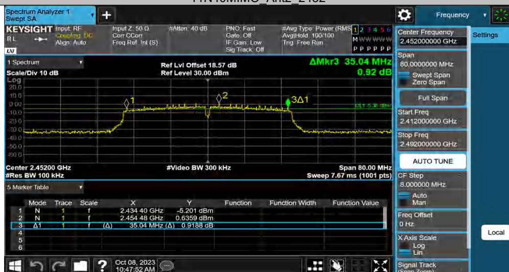
11N40MIMO Ant2 2452
