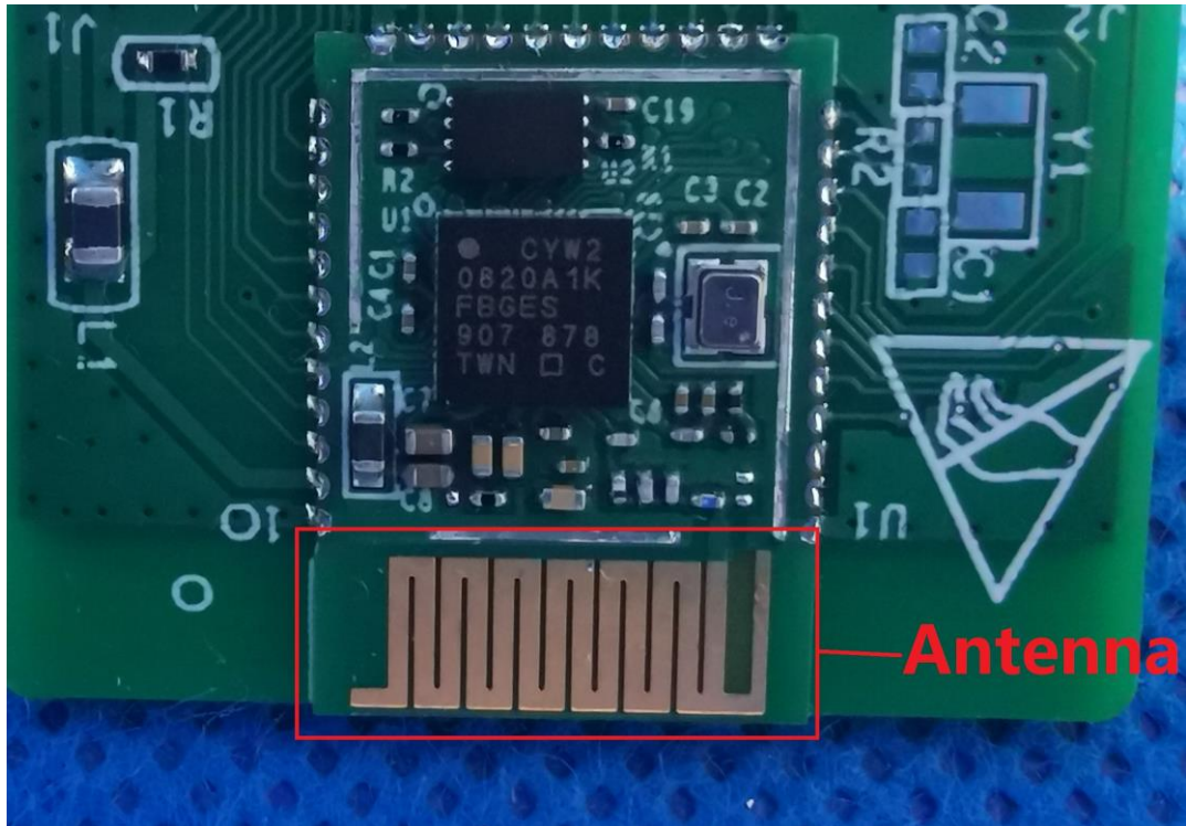
(1) EUT Photo (CYBT-243068-02)
