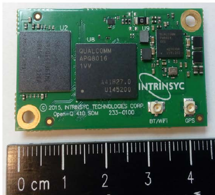
Bottom (RF Shield Removed) and Top Side of Module
