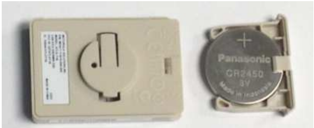
Figure 6 Battery Tray
