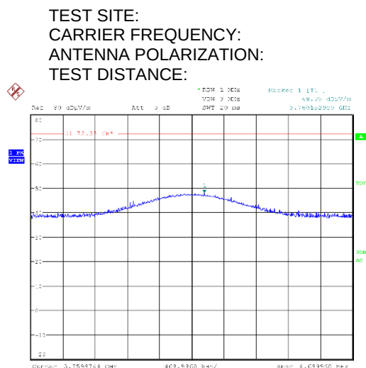
Plot 7.4.18 Radiated emission measurements at the 8 th harmonic
