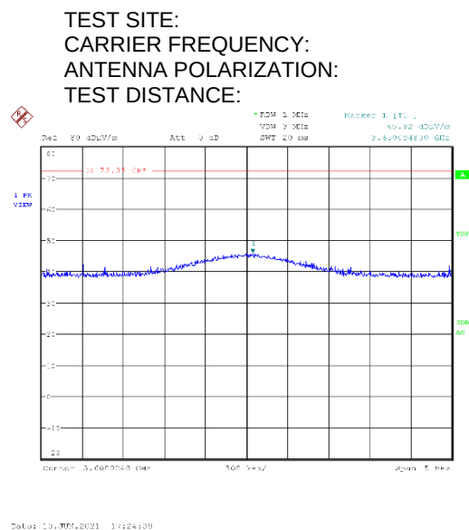
Plot 7.4.16 Radiated emission measurements at the 8 th harmonic
