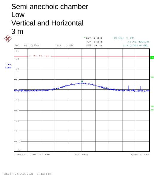
Plot 7.4.16 Radiated emission measurements at the 8 th harmonic
