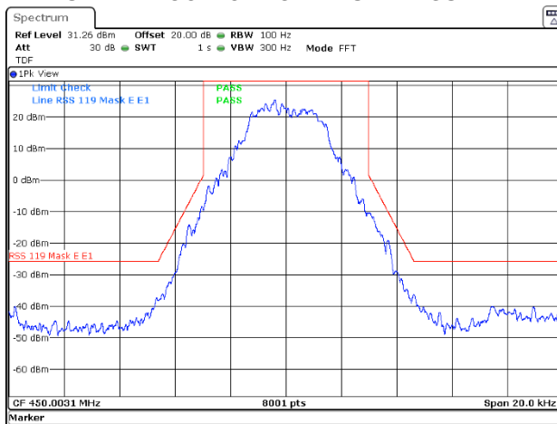
lot 7.3.5 Emission mask test results at mid carrier frequency RSS-119
