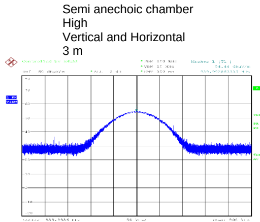
Plot 7.4.12 Radiated emission measurements at the 2 nd harmonic
