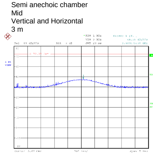
Plot 7.4.17 Radiated emission measurements at the 8 th harmonic
