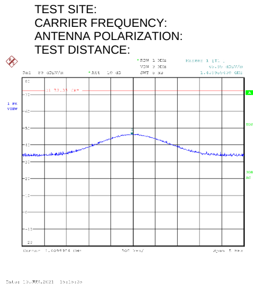
Plot 7.4.15 Radiated emission measurements at the 3 rd harmonic
