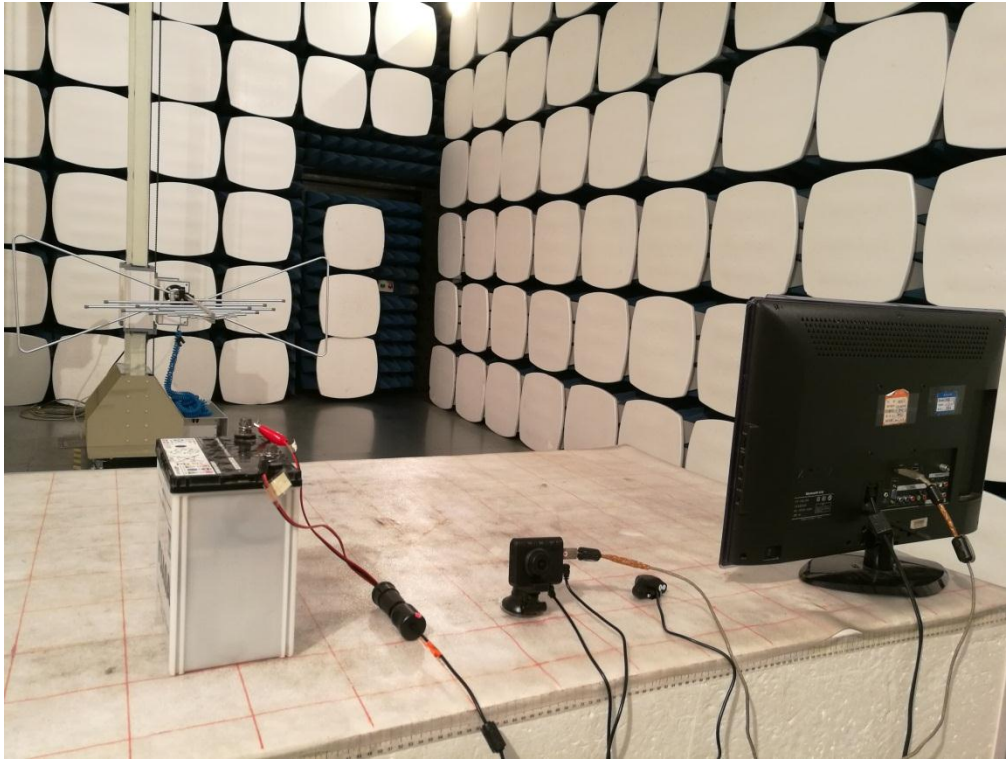
Radiated Emission(For DC 12V) Below 1GHz
