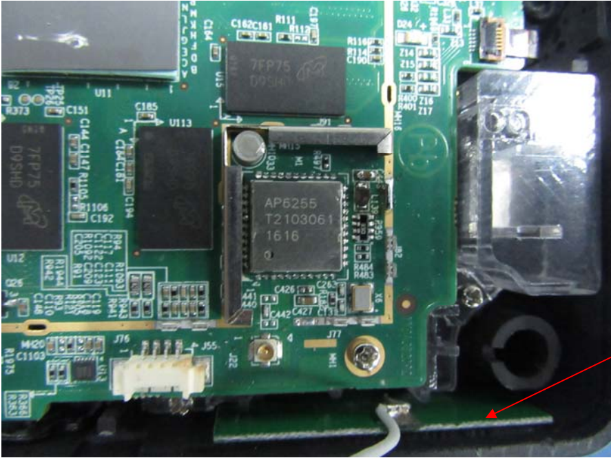
EUT_WLAN & Bluetooth RF Module View
