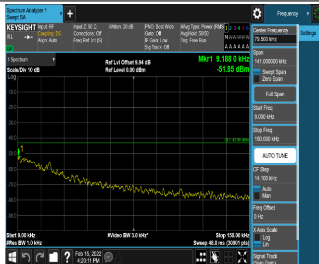
Band25-10MHz-QPSK-26640-1-0-High-0.009-0.15--51.85-PASS
