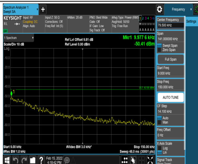
Band25-10MHz-16QAM-26365-1-0-Low-0.009-0.15--50.41-PASS
